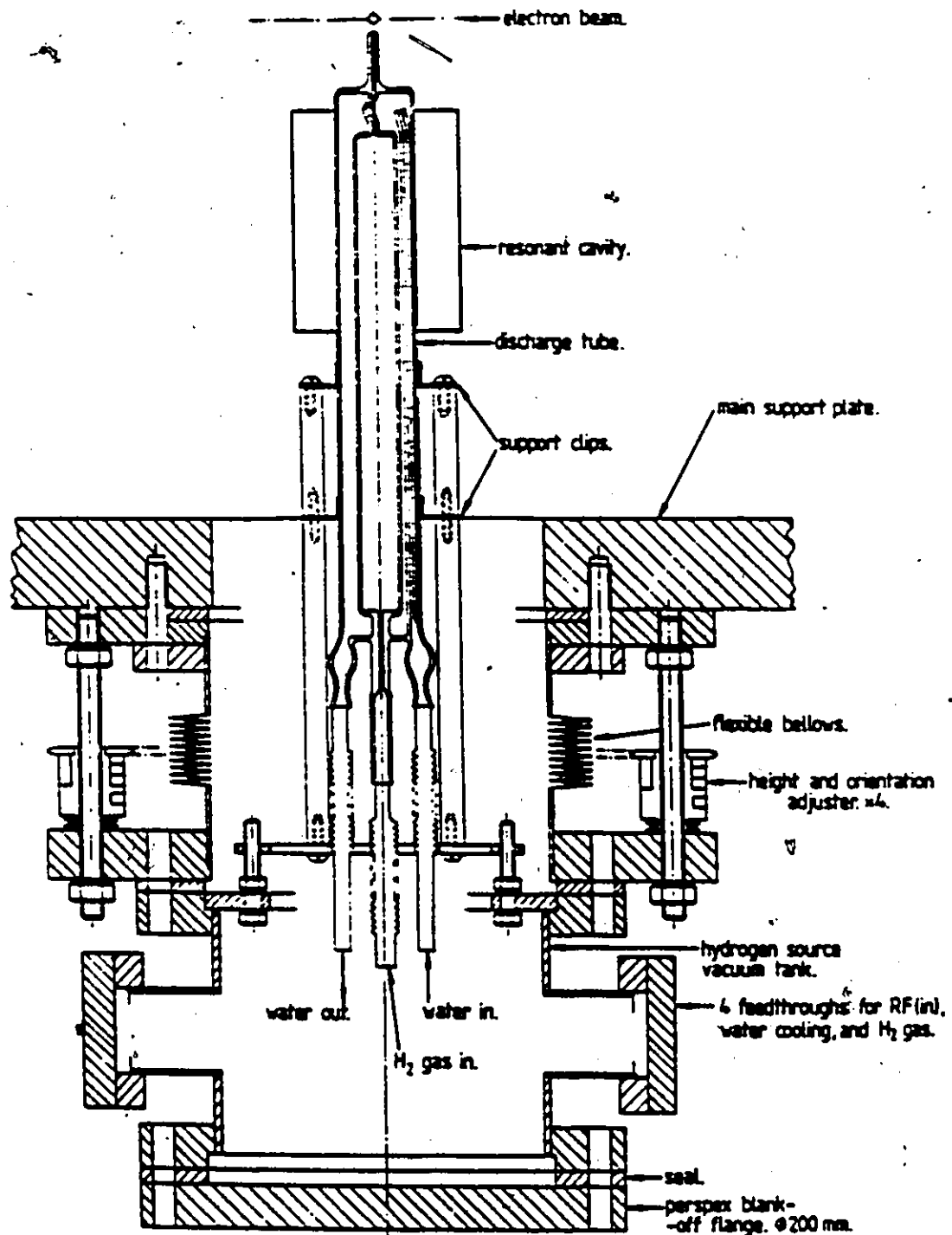
Figure 49: Illustrated is the complete rf-discharge source including its vacuum tank and external connections.
