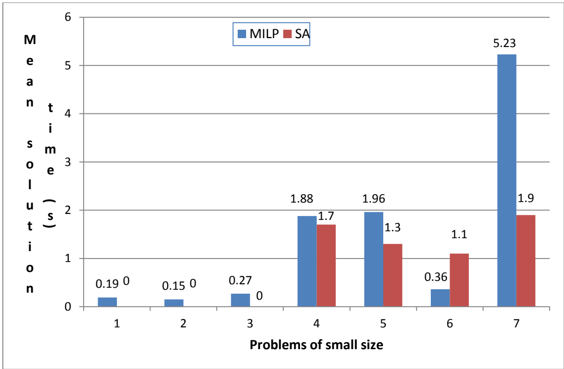
Figure 17: Comparison of mean solution time required for MILP model and SA algorithm for problems of small size
