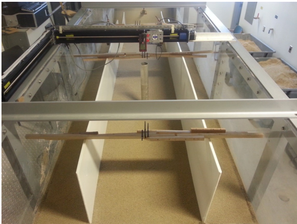
Figure 3.3. Experimental set-up
