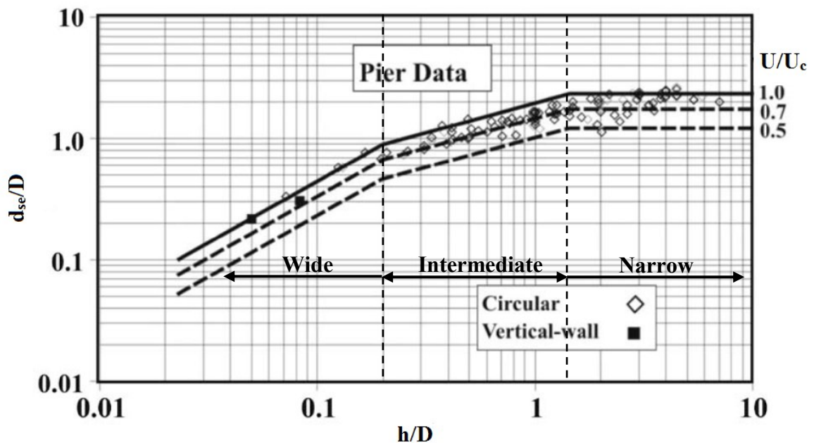
Figure 2.3. Graphical relationship between d_{sc}/D and h/D based on U/U_c (Melville and Coleman, 2000: used with permission from Water Resources Publications)
