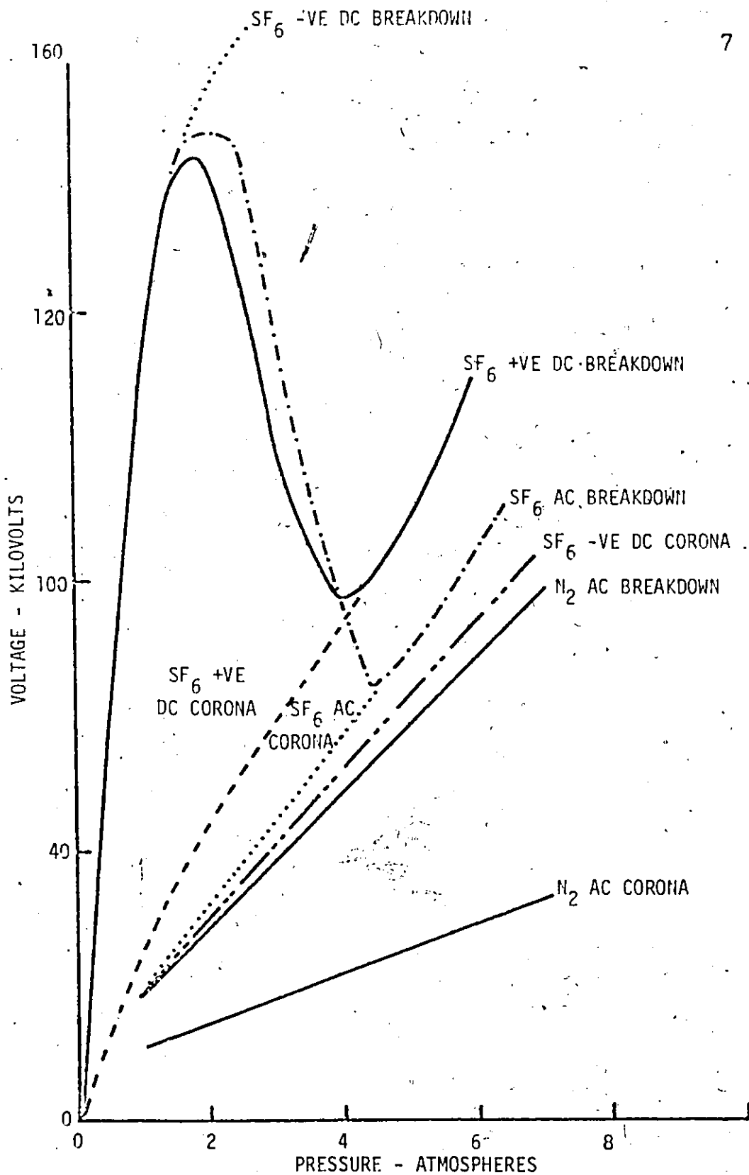
FIGURE 1.2. BREAKDOWN AND CORONA ONSET VOLTAGES OF A 1/16 INCH DIAMETER ROD-PLANE GAP OF 1.0 INCH LENGTH (FROM REFERENCE 5).
