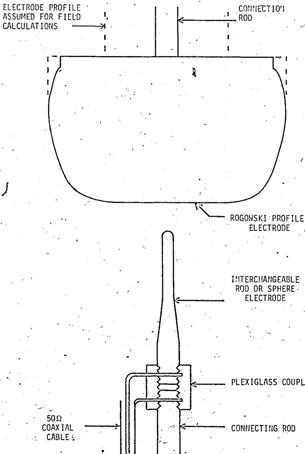
FIGURE 2.2. ELECTRODE ASSEMBLY.
