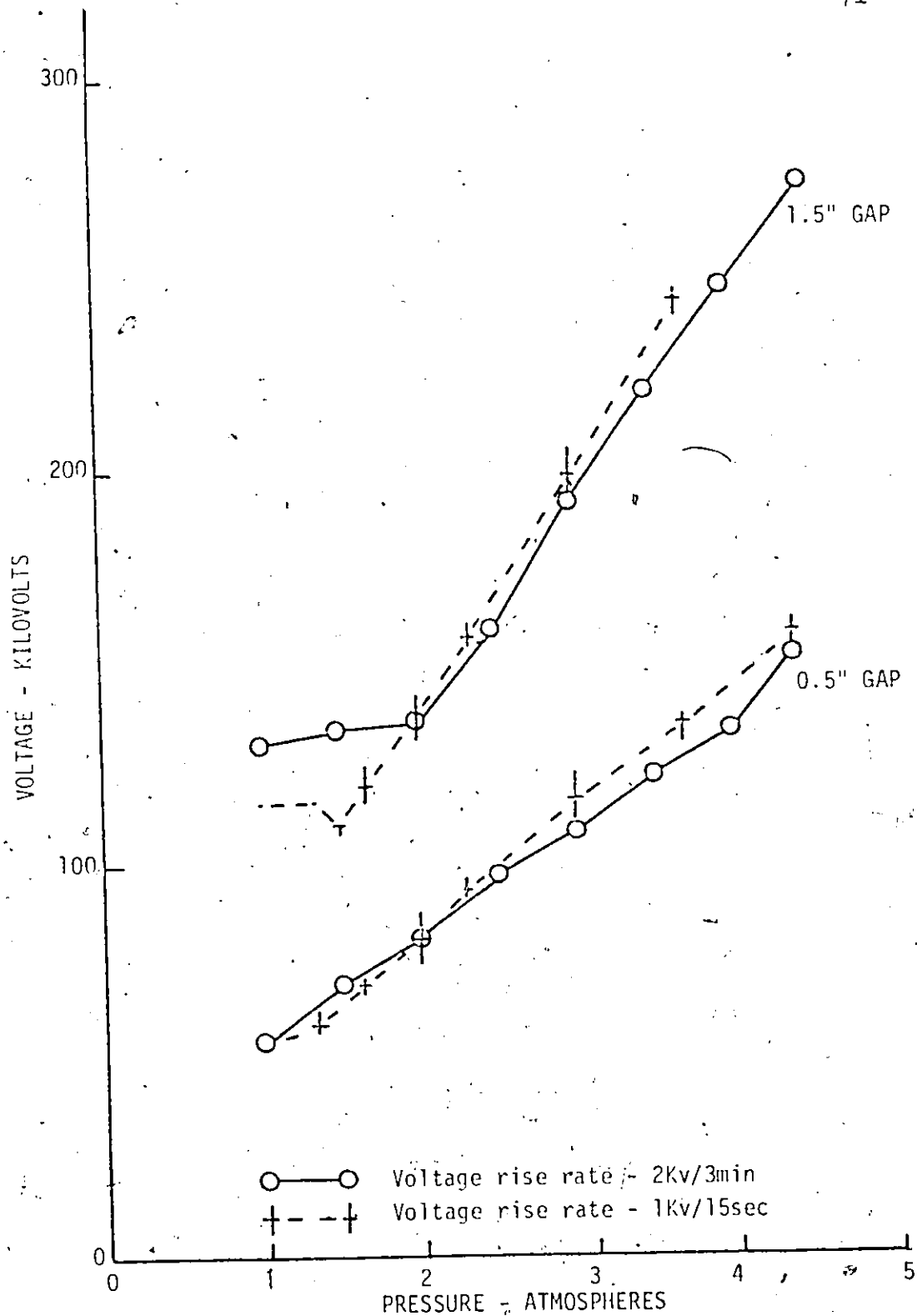
FIGURE 4.11. COMPARISON OF TEST RESULTS OBTAINED IN TWO DIFFERENT TEST SERIES OF A 1/4 INCH DIAMETER ROD-PLANE GAP.
