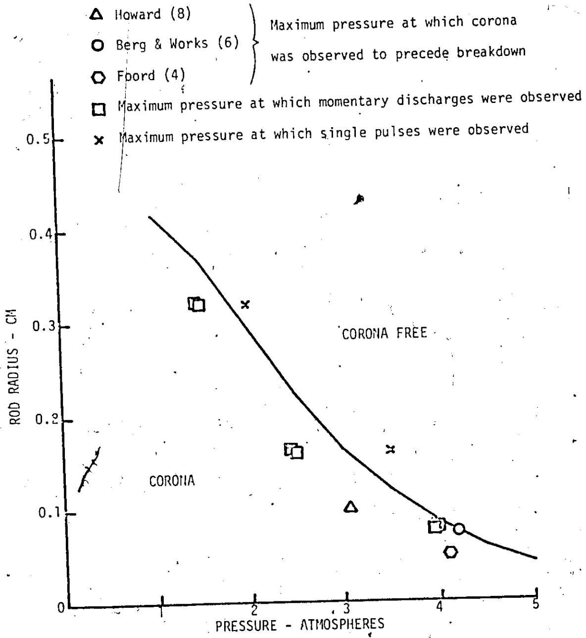
FIGURE 6.7. THEORETICAL CALCULATIONS AND EXPERIMENTAL MEASUREMENTS OF THE ONSET PRESSURE OF CORONA FREE BREAKDOWN IN SF 6 .
