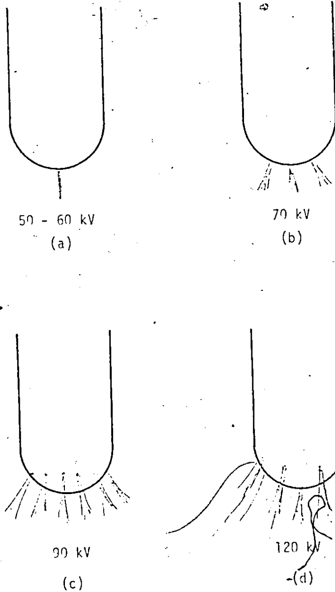
FIGURE 3.7. VISUAL APPEARANCE OF CORONA DISCHARGES IN \text{SF}_6 AT THE TIP OF A 1/16 INCH DIAMETER ROD, AT A GAS PRESSURE OF 1 ATMOSPHERE.
