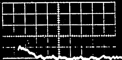
3. 1 \mu AMP/DIV, 1 \mu SEC/DIV P - 1 ATM, ELECTRODE 1/8 - 1/2 V = 27 KV
