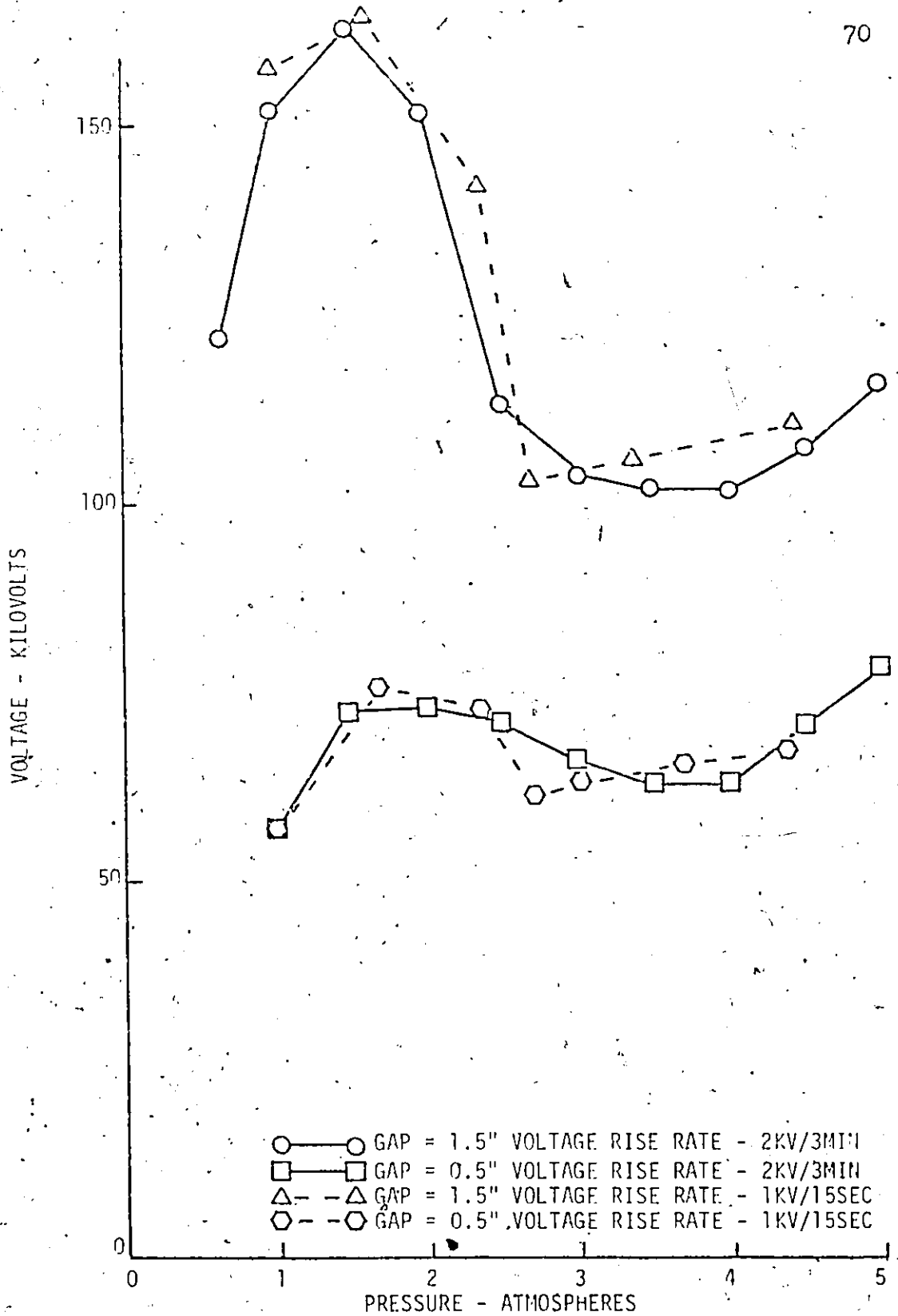
FIGURE 4.10. COMPARISON OF TEST RESULTS OBTAINED IN TWO DIFFERENT TEST SERIES OF A 1/16 INCH DIAMETER ROD-PLANE GAP.
