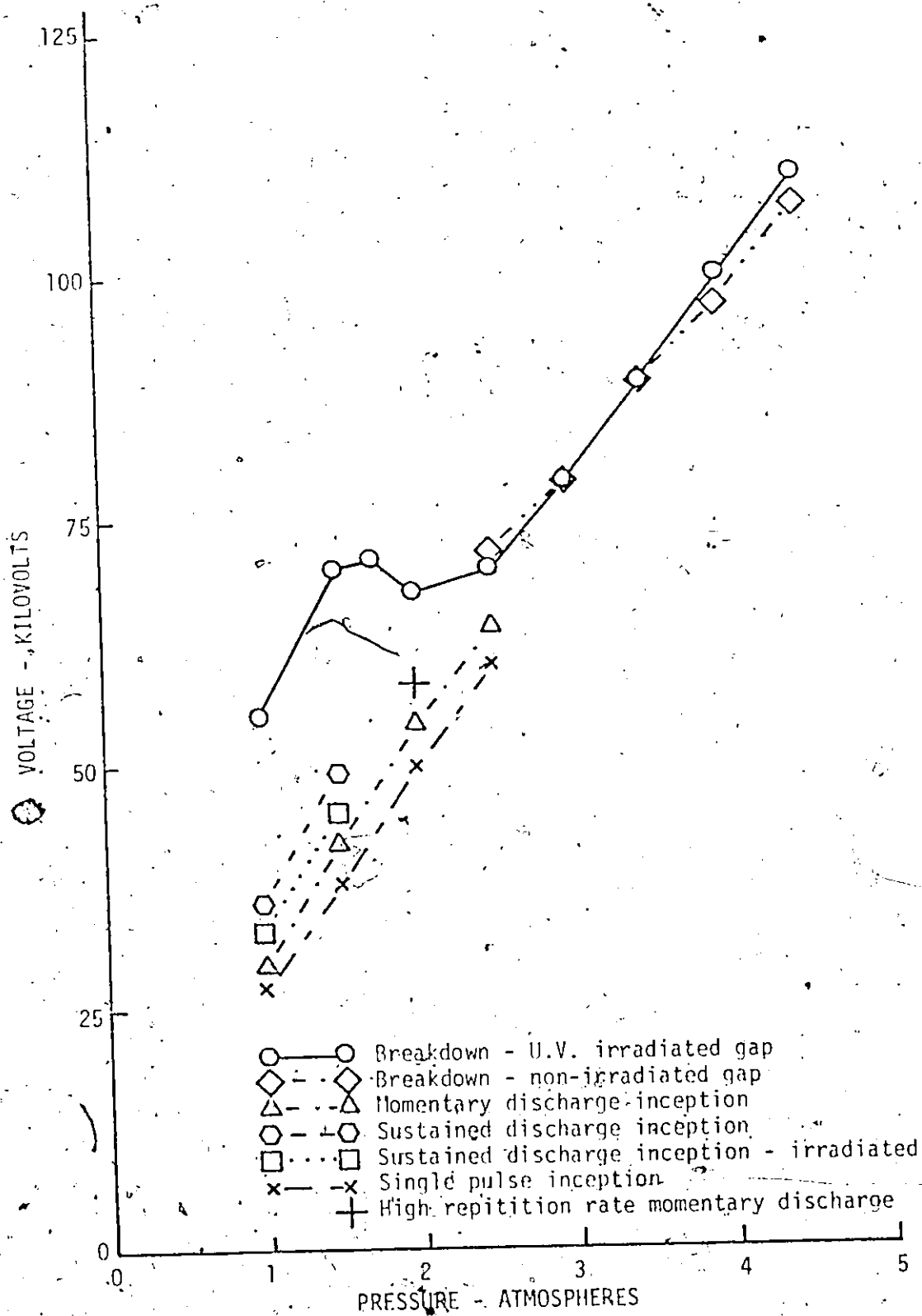
FIGURE 4.3. BREAKDOWN AND CORONA DISCHARGE INCEPTION VOLTAGES OF A 1/8 INCH DIAMETER ROD-PLANE GAP OF 0.5 INCH LENGTH.
