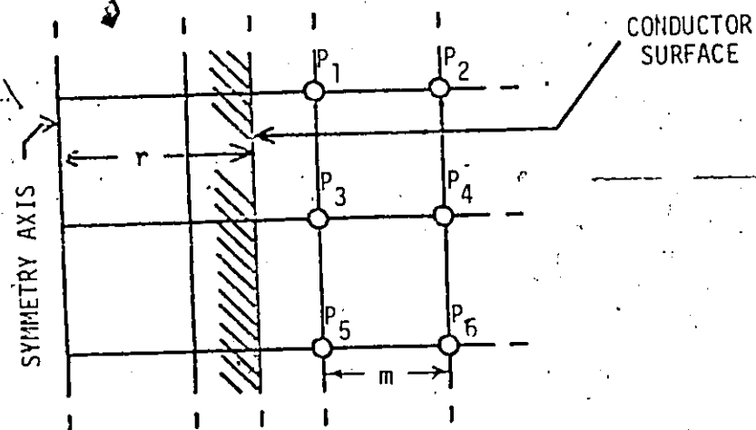
FIGURE 6.3. MESH POINTS ADJACENT TO A DIRICHLET BOUNDARY.
