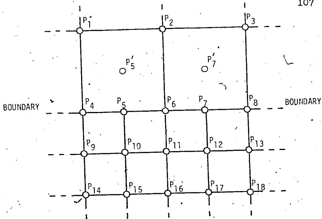
FIGURE 6.2. BOUNDARY BETWEEN TWO AREAS OF DIFFERENT MESH LENGTH.
