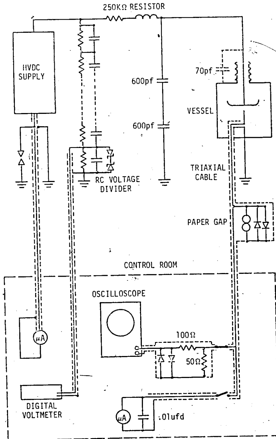
FIGURE 2.5 SCHEMATIC OF HIGH VOLTAGE AND MEASUREMENT CIRCUITRY.
