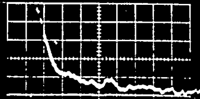
4. 1 \mu AMP/DIV, 1 \mu SEC/DIV P - 1 ATM, ELECTRODE 1/8 - 1/2 V = 27 KV
