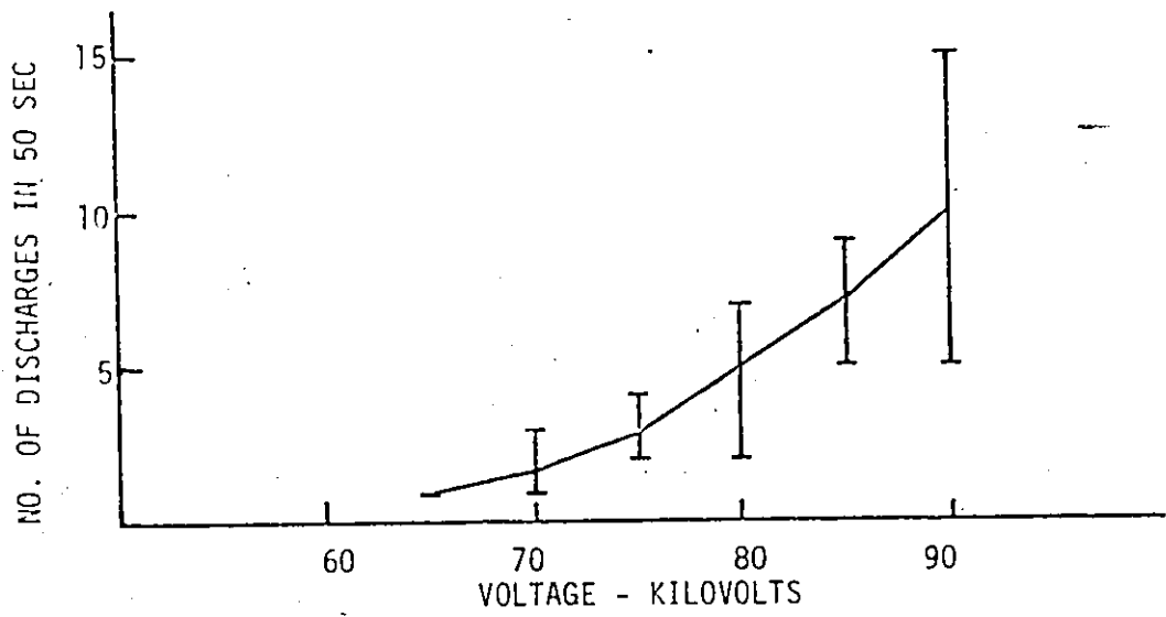
FIGURE 3.3. THE RELATIONSHIP BETWEEN APPLIED VOLTAGE AND THE MAGNITUDE, THE DURATION, AND THE REPETITION RATE OF MOMENTARY DISCHARGES IN A 1/16 INCH DIAMETER ROD-PLANE GAP OF 1.5 INCHES LENGTH, AT A GAS PRESSURE OF 2.7 ATMOSPHERES. BREAKDOWN OCCURRED AT 100 KV.
