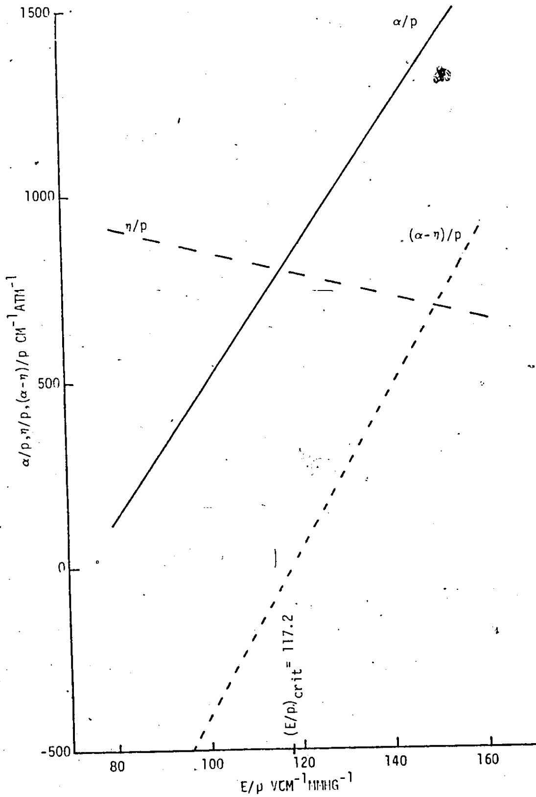
FIGURE 6.4. IONIZATION AND ATTACHMENT COEFFICIENTS OF \text{SF}_6 .
