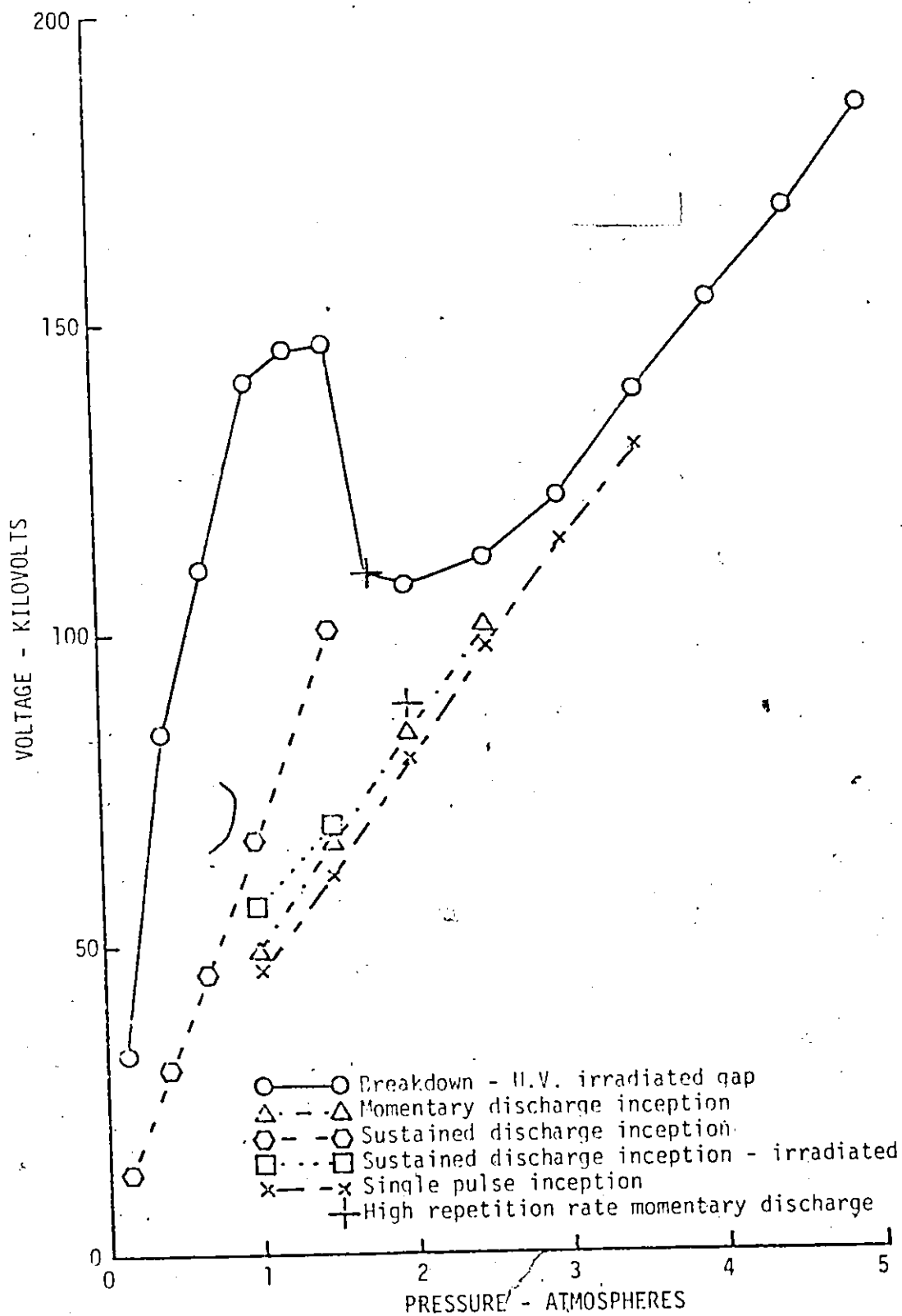
FIGURE 4.5. BREAKDOWN AND CORONA DISCHARGE INCEPTION VOLTAGES OF A 1/8 INCH DIAMETER ROD-PLANE GAP OF 1.5 INCHES LENGTH.
