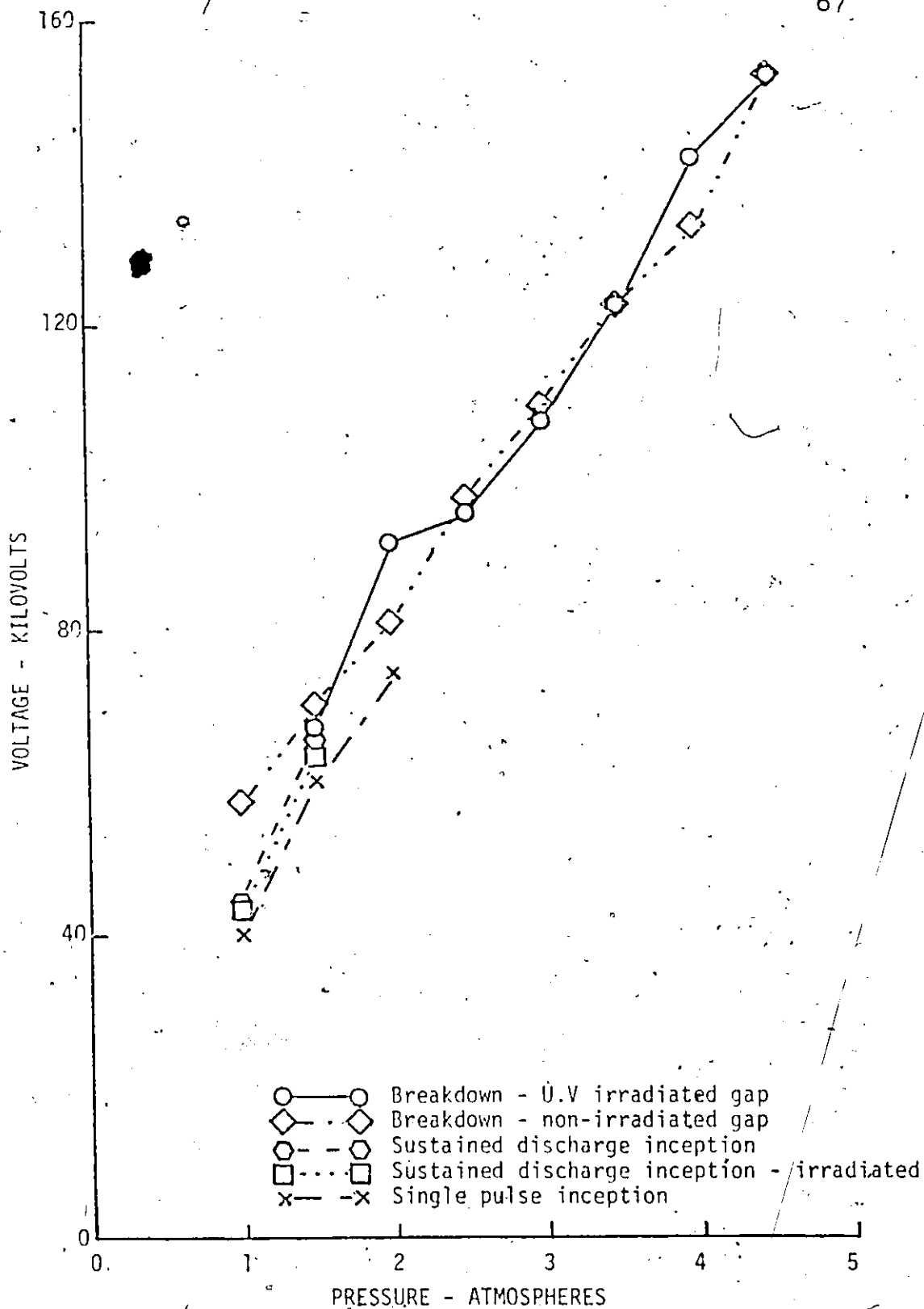
FIGURE 4.7. BREAKDOWN AND CORONA DISCHARGE INCEPTION VOLTAGES OF A 1/4 INCH DIAMETER ROD-PLANE GAP OF 0.5 INCH LENGTH.
