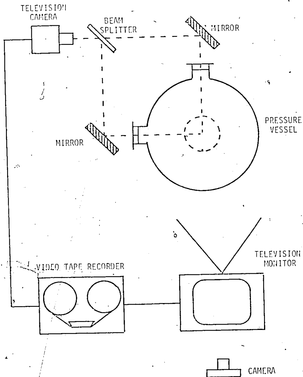
FIGURE 4.12. EXPERIMENTAL SETUP FOR THE ANALYSIS OF SPARK TRAJECTORIES.
