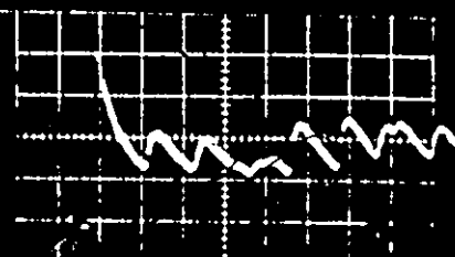
6. 4 \mu AMP/DIV, 1 \mu SEC/DIV P - 1 ATM, ELECTRODE 1/8 - 1/2 V = 29 KV
