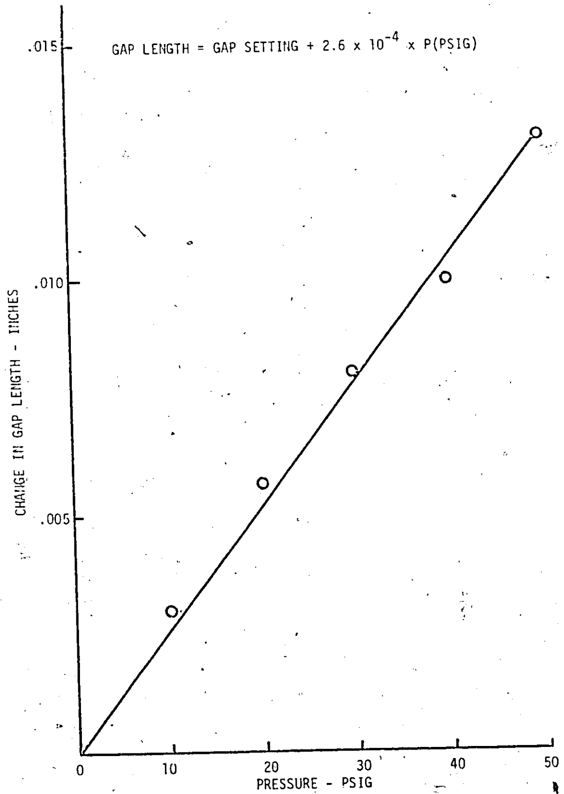
FIGURE 2.3. EFFECT OF GAS PRESSURE ON GAP LENGTH.
