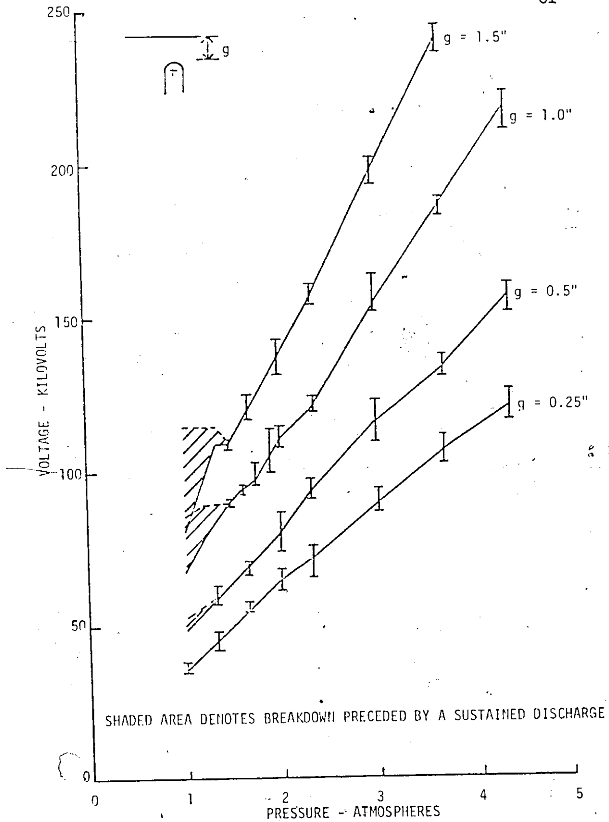
FIGURE 4.2. BREAKDOWN AND CORONA ONSET VOLTAGES OF A 1/4 INCH DIAMETER ROD-PLANE GAP.
