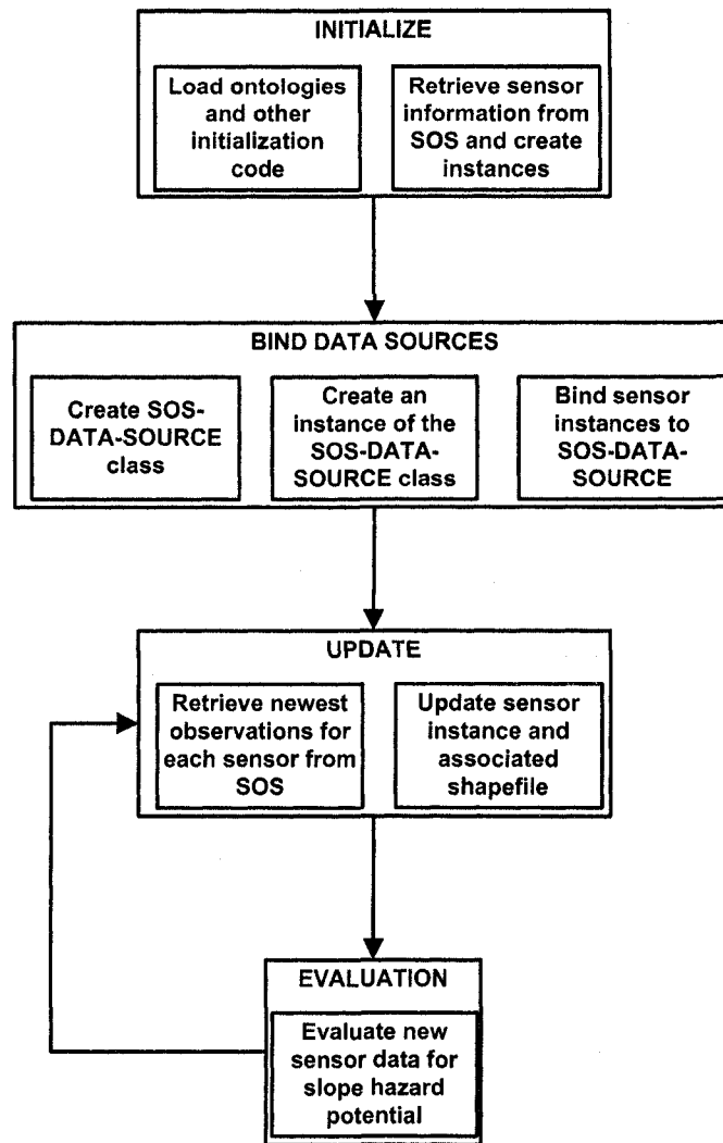
Figure 13 - Expanded version of the REASON evaluation loop
