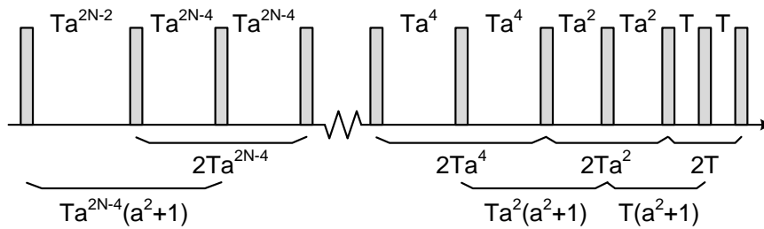
Figure 2-7. eChirp train structure
