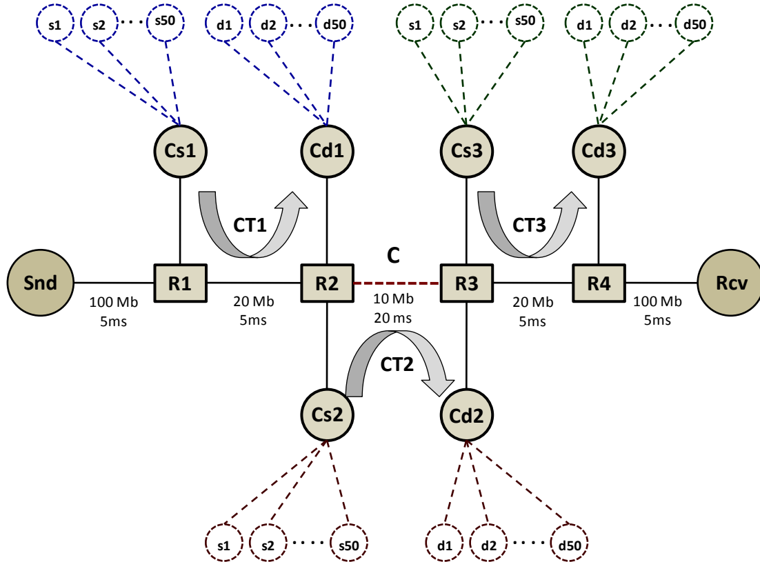
Figure 4-6. Simulation topology for Pre-bottleneck and Post-bottleneck experiments
