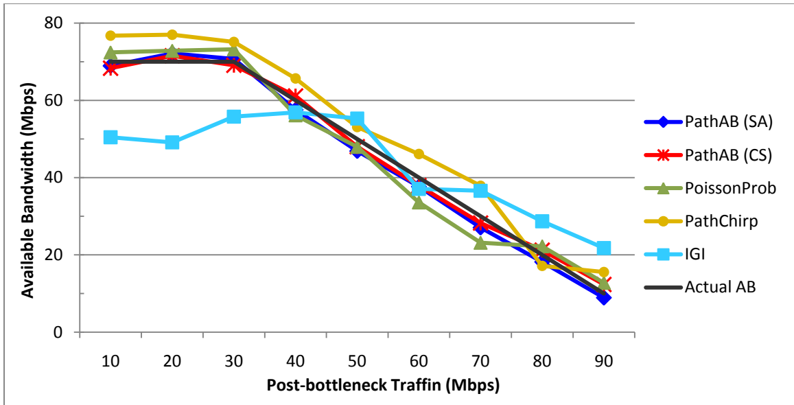
Figure 4-16. Comparison of average estimated AB by different algorithms in 100Mbps multi-hop path under post-bottleneck traffic
