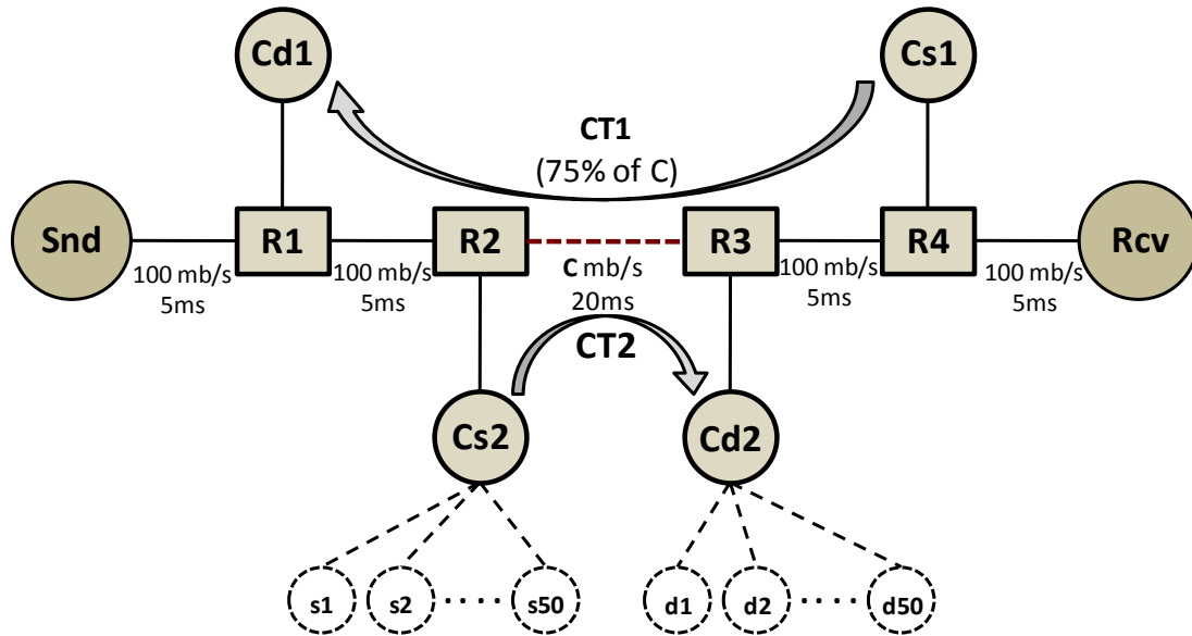
Figure 4-1. Network model for single bottleneck experiments
