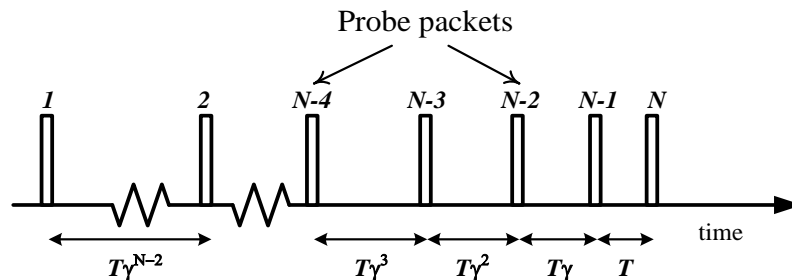
Figure 3-1. Exponentially spaced probing train
