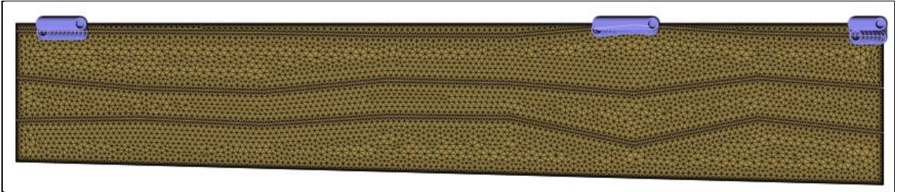
Figure 3.3a: Boundary condition for mass-transport showing the location of the contaminant source in the south-north model
