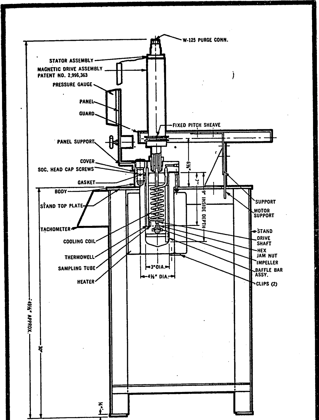
FIGURE IV-2 STANDARD ONE LITER AFP-1005 PACKLESS AUTOCLAVE ( Autoclave Eng. )
