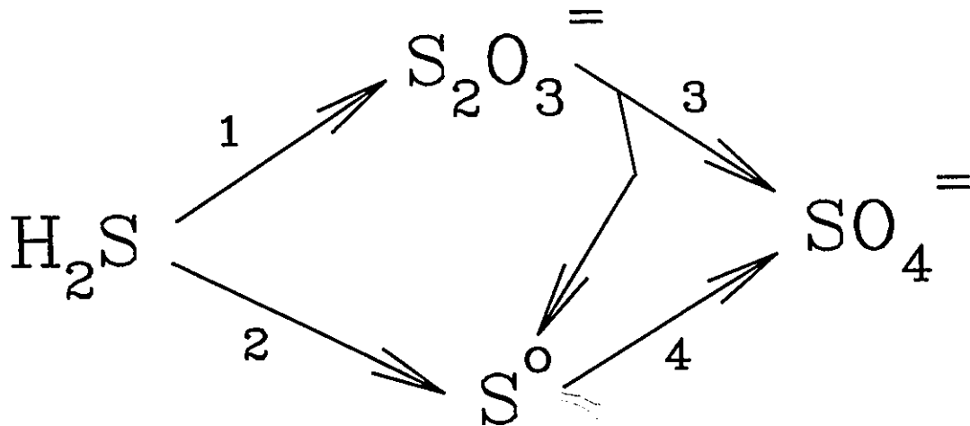
FIGURE 5.5 Simplified reaction pathways
