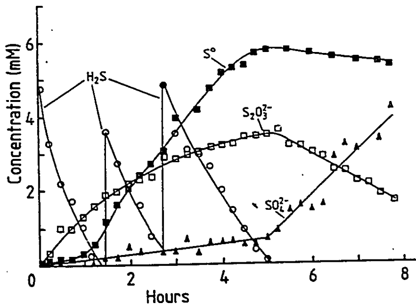
FIGURE 5.3 Concentrations of \text{H}_2\text{S} (O), \text{S}_2\text{O}_3^{2-} ( \square ), \text{S}^0 ( \blacksquare ), and \text{SO}_4^{2-} ( \blacktriangle ) as functions of time in a batch culture (Brune, 1989)
