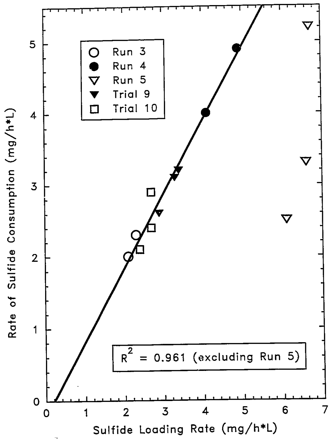
FIGURE 4.16 Sulfide consumption and loading
