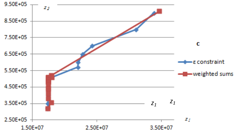
Figure 3.4. Trade-off surfaces for the test problem 2: (a) weighted sums method, (b) \epsilon -constraint method, (c) weighted sums and \epsilon -constraint methods
