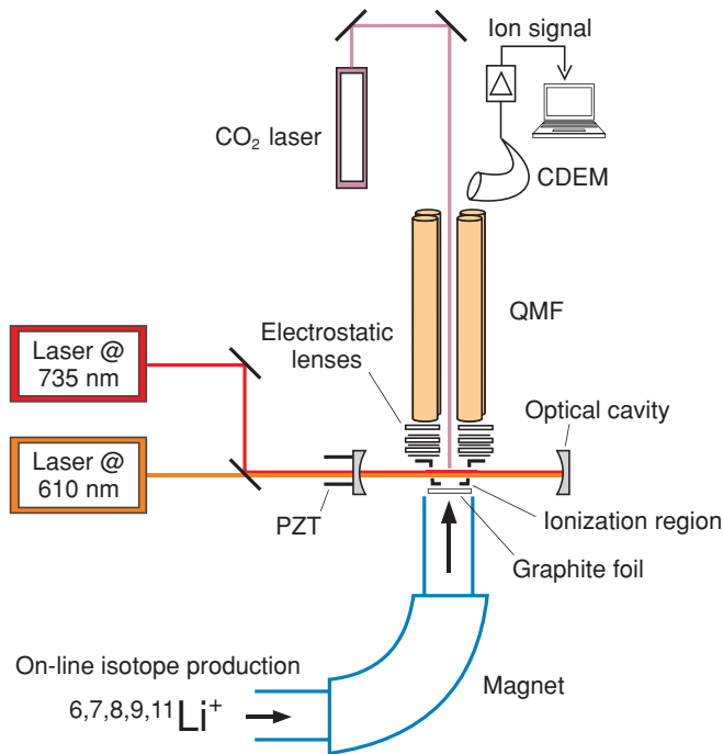
FIG. 2. (Color online) Experimental setup to measure the 2s^2S_{1/2} \rightarrow 3s^2S_{1/2} electronic transition in lithium. CDEM, continuous dynode electron multiplier; QMF, quadrupole mass filter; PZT, piezoelectric transducer.
