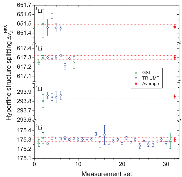
FIG. 16. (Color online) Results of all hyperfine splitting measurements in the 2s^2S_{1/2} \rightarrow 3s^2S_{1/2} transition of Li isotopes as obtained during the off-line and on-line beam times at GSI and TRIUMF. For {}^7\text{Li} , additional off-line measurements were performed at GSI after the TRIUMF measurements using a frequency comb for laser frequency stabilization [27]. These results are shown as the rightmost GSI datapoint and are in good agreement with previous data. Plotted are the measured two-photon frequency intervals \Delta\nu_A^{\text{HFS}} (twice the Ti:sapphire laser frequency difference) between F \rightarrow F transitions for F = I - 1/2 and F = I + 1/2 . Each data point (circle) is the average of 10–20 measurements. The rightmost data point (solid circle) represents the weighted average. For their uncertainties, see the caption of Table X.
