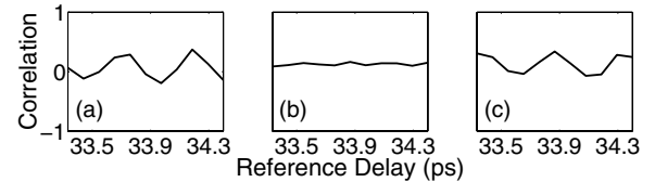
FIG. 3. Two-state wave packet correlations. (a) In the absence of a HCP, the 27p - 32p correlation is strong; the phase relationship is well defined and easily read. (b) T_1 = 7 ps. The operation of the HCP moves phase information into the 31d and 32s states, and that phase information becomes unreadable. (c) T_2 = 14.2 ps. Application of a second HCP at a later delay recovers phase information in the 32p state.
