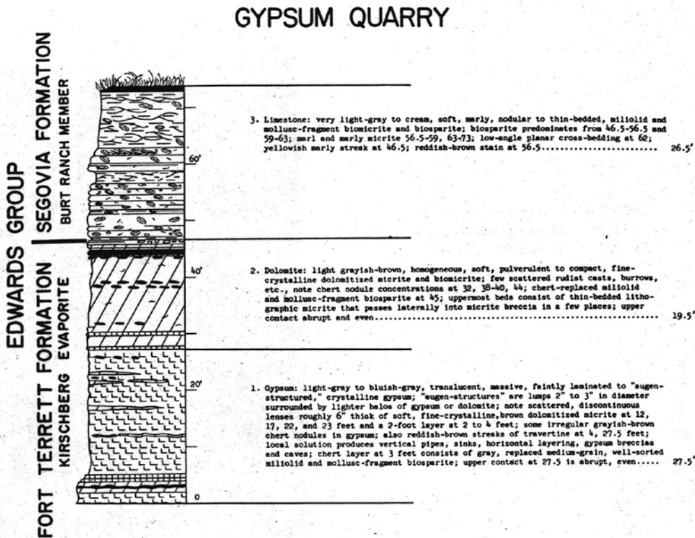
Figure 10 Stratigraphic section for the Cretaceous units present in the Gypsum Mine. Note that the gypsum is present in the Fort Terrett Formation of the Edwards Group. Section from Barns, Kaiser, Maclay and Young 1976 p. 14.
