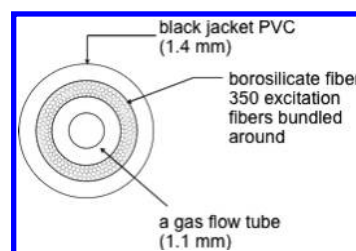
Figure 9. A schematic cross-section picture of the hollow-core fiber optic, in which \sim 350 excitation fibers surround the Teflon inner flow tube coaxially.
