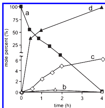
Figure 7. Reaction profile of fiber optic delivering light and oxygen to the probe tip (a) percent sensitizer bioconjugate 1, (b) percent surface-bound dioxetane 2, (c) percent 3 photoreleased into toluene- d_8 at room temperature, and (d) percent 3 photoreleased into petrolatum at 65 °C.
