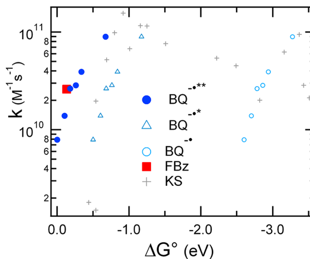
Figure 6. Rate constants for reaction of solvated electrons e^-_{\text{s}} in THF with substituted benzoquinones (RBQ) as a function of free energy change, \Delta G^\circ , for attachment to form ground state radical anions, \text{RBQ}^{\bullet-} (blue \circ ). These rates are replotted vs \Delta G^\circ + 2.6 \text{ eV} to estimate energetics for reaction to form the \pi^* excited states \text{RBQ}^{-\bullet\bullet} (blue \bullet ), and vs \Delta G^\circ + 2.1 \text{ eV} for the n\pi^* \text{RBQ}^{-\bullet\bullet} (excited states) (light blue \triangle ). The measurements are compared with rate constants for e^-_{\text{s}} with fluorobenzene (red \blacksquare ), 35 and a series of molecules by Kadhum and Salmon (KS, +). 47 Free energy changes for the substituted benzoquinones (denoted BQ) and the KS data were estimated from redox potentials and Kukhareenko's determination for the solvated electron. 64
