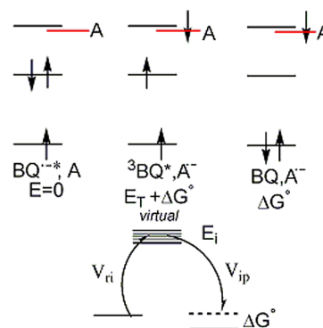
Figure 5. Schematic orbital diagram (upper) and state diagram (lower) for electron transfer from BQ^{\bullet-} to an acceptor, A. The two-electron change is depicted to be accomplished first by transfer of an electron to the acceptor to create a high-energy (virtual) intermediate (the configuration in the middle of the three shown). This is followed by a second virtual step that moves the now unpaired electron to the lowest orbital shown. The state diagram shows ET to occur from the reactants to the products, lower by \Delta G , via interaction with a high-energy virtual intermediate having an energy well above that of the reactants. The energy of the intermediate, relative to that of the reactants, E_i , is approximately the triplet energy ( E_T ) of BQ + \Delta G^\circ (note that \Delta G^\circ is usually negative).
