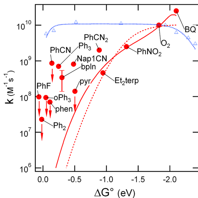
Figure 3. Bimolecular rate constants for electron transfer from \text{BQ}^{\bullet-} to electron acceptors in THF at 296 K. The rate constants were measured by observing \text{BQ}^{\bullet-} ground state recovery at 450 nm after excitation at 420 nm in solutions of 5 mM BQ partially reduced by NaK in the presence of \text{C}_{222} . The observed rate constants are compared with earlier data. A fit (red dashed line) to a single-step electron transfer mechanism (eq 6) having a constant electronic coupling, V = 223 \text{ cm}^{-1} , does not describe the data well, even with large reorganization energies, \lambda_s = 0.6 and \lambda_v = 2.9 \text{ eV} (see Discussion). Equation 7 includes transition of a second electron in simple description, predicting that V varies with \Delta G^\circ , yields a slightly improved fit (solid line). This description, described in Discussion, requires a much smaller \lambda_v = 0.85 \text{ eV} . For comparison rates of bimolecular electron transfer from anions of biphenyl are shown (blue \Delta ). 38
