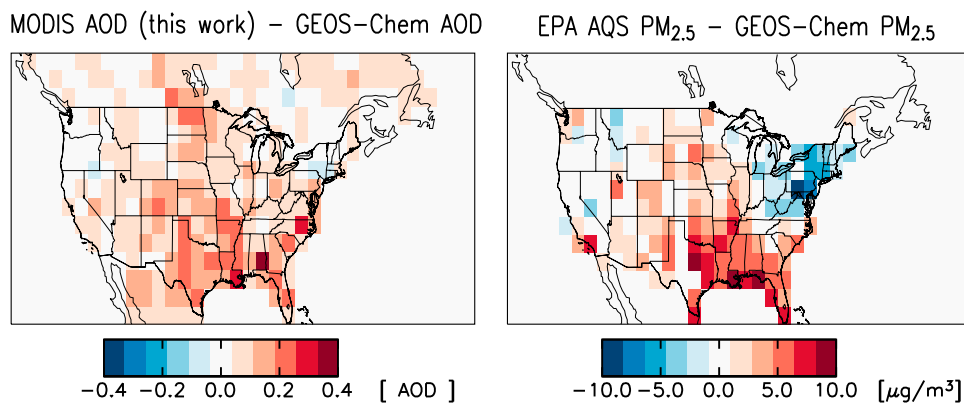
Figure 16. GEOS-Chem model bias relative (left) to our MODIS AOD retrieval and (right) to the EPA-AQS surface \text{PM}_{2.5} network. Values are averages for the ICARTT period (06 July to 14 August 2004).
