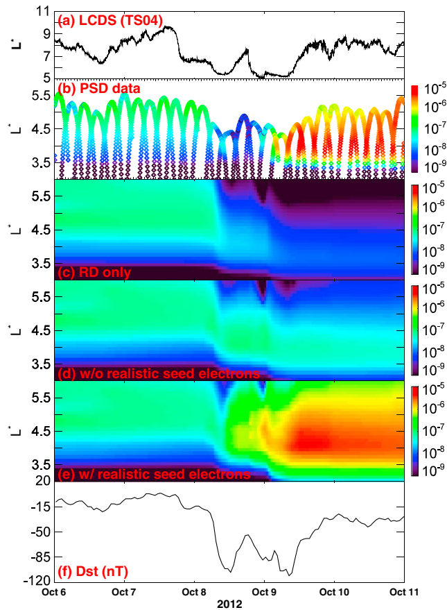
Figure 1. Electron PSD data (in units of c/\text{MeV}/\text{cm}^3 ) and simulation results at \mu = 1279 \text{ MeV}/\text{G} and K = 0.115 \text{ G}^{1/2} R_E for the October 2012 storm, with (a) last closed drift shell calculated using TS04 model; (b) PSD data from Van Allen Probes; (c–e) model results with “RD only,” “RD + Hiss + Chorus” without realistic electron seed population, and “RD + Hiss + Chorus” with realistic electron seed population, respectively; and (f) Dst index.
