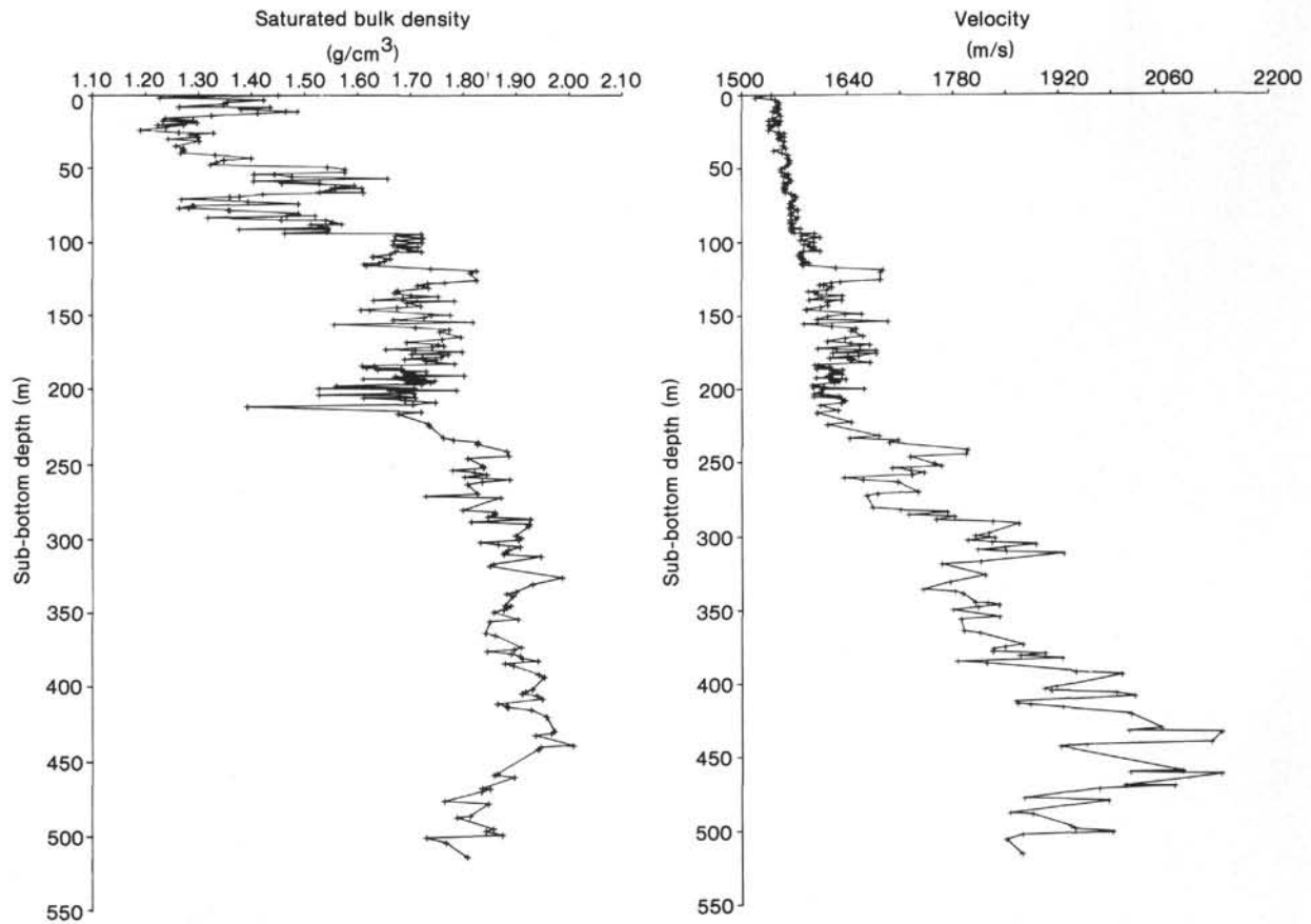
Figure 4. Laboratory-measured saturated bulk density and sonic velocity versus sub-bottom depth for DSDP Site 574.
