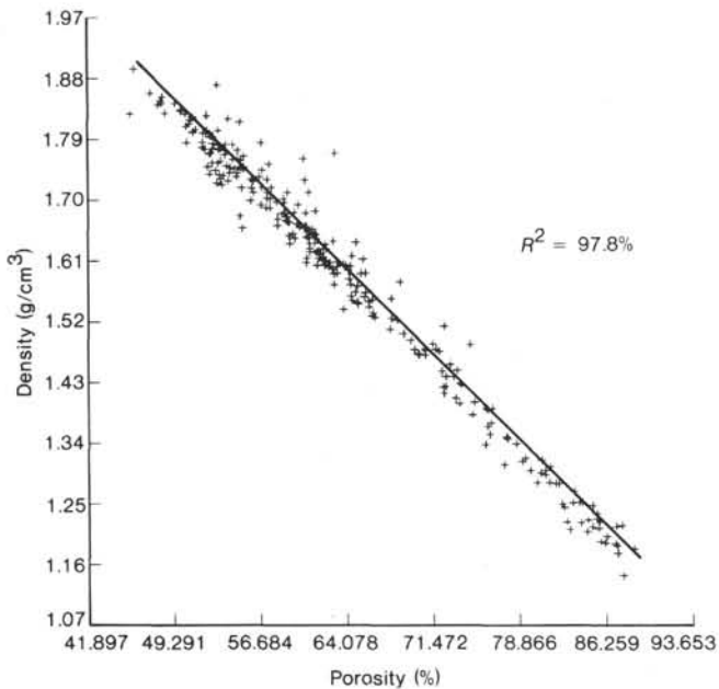
Figure 6. Regression of saturated bulk density against porosity for DSDP Site 574. R^2 = correlation coefficient.
