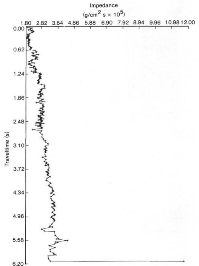
Figure 10. Impedance versus traveltime, DSDP Site 574.
