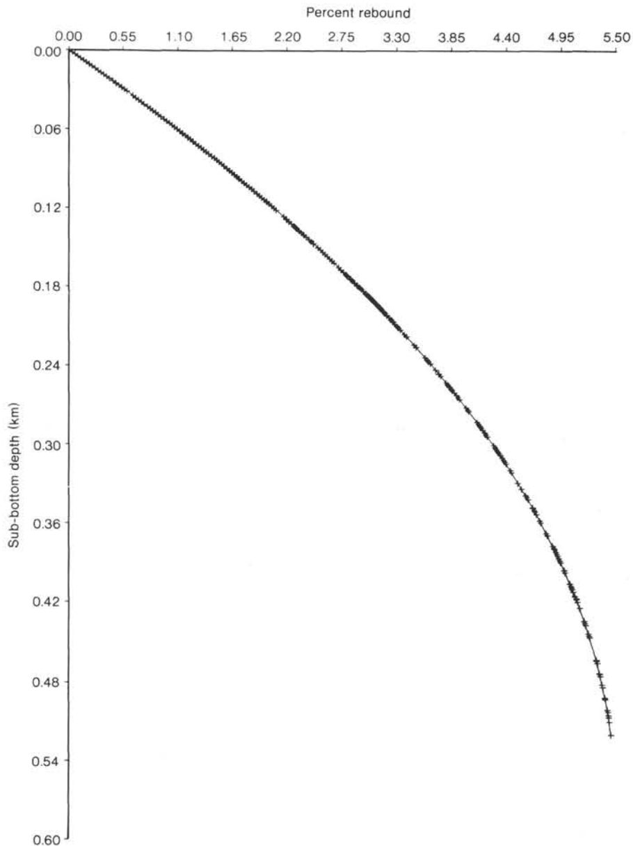
Figure 5. Calculated percent porosity rebound versus sub-bottom depth for DSDP Site 574.
