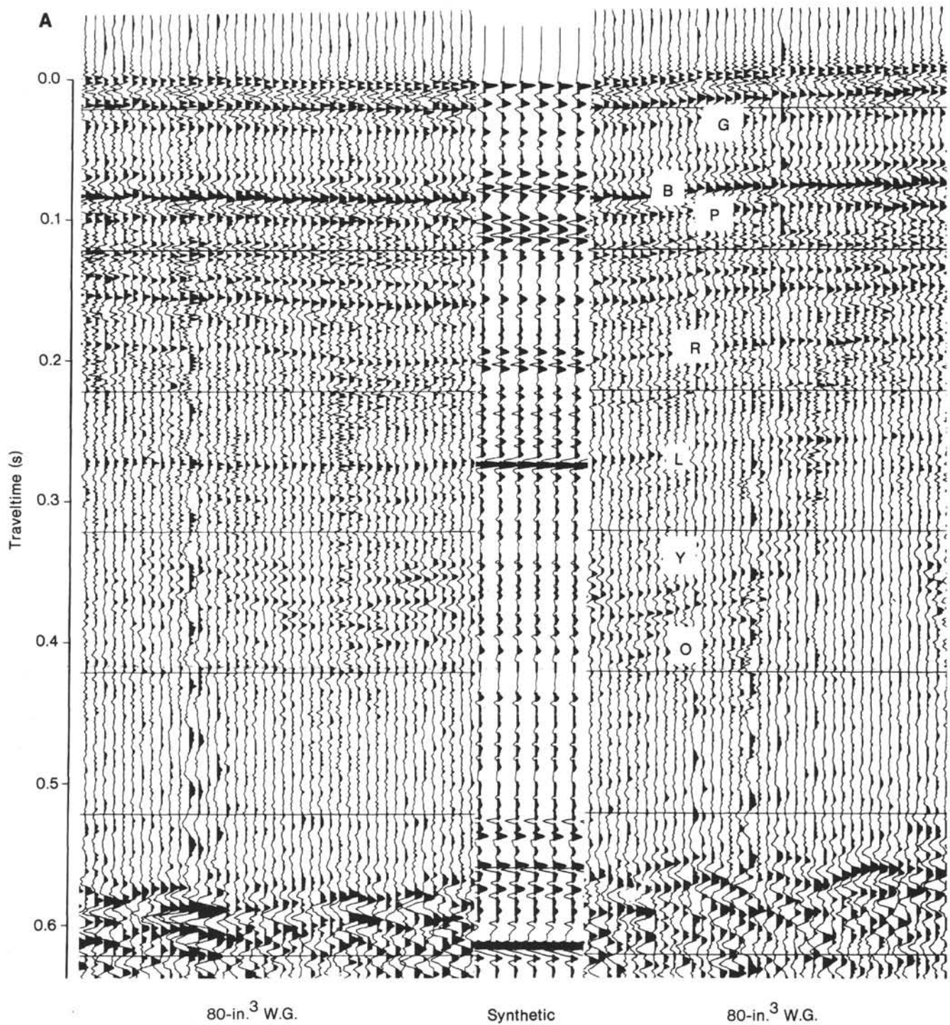
Figure 13. Comparisons of field data with synthetic seismograms. W.G. = field watergun record. A. Deconvolved source, no mix. B. Deconvolved source, 3-trace mix. C. Raw source, no mix. D. Raw source, 3-trace mix.
