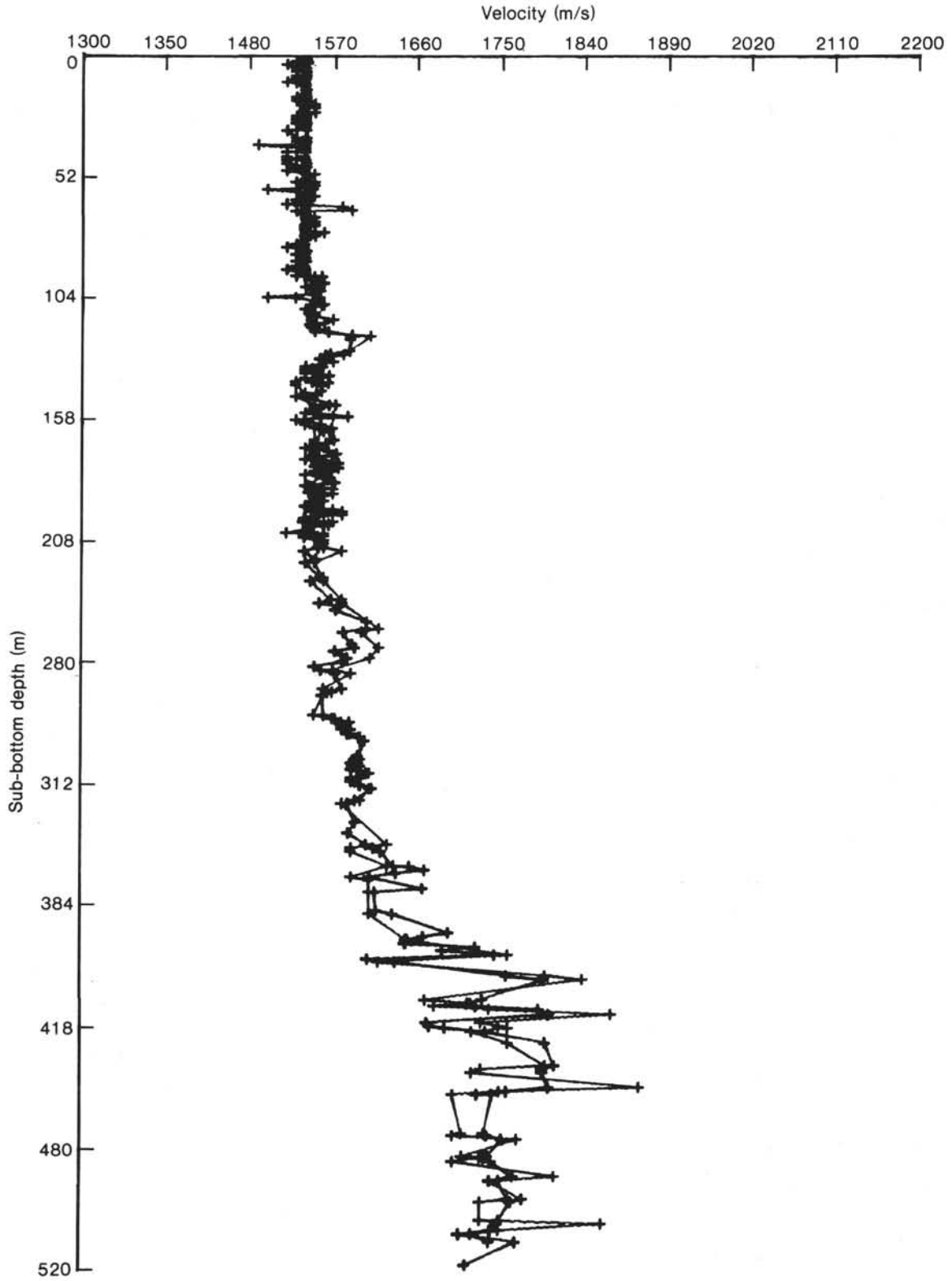
Figure 8. Predicted (from porosity) laboratory velocity versus sub-bottom depth and measured laboratory velocity versus sub-bottom depth, DSDP Site 574.
