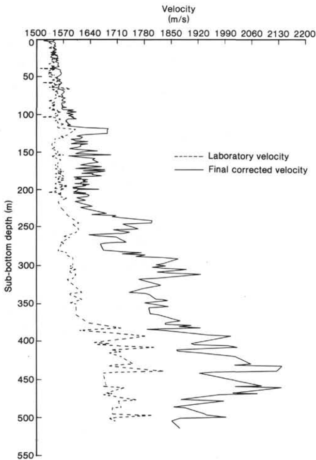
Figure 9. Laboratory velocity and final corrected velocity versus sub-bottom depth.
