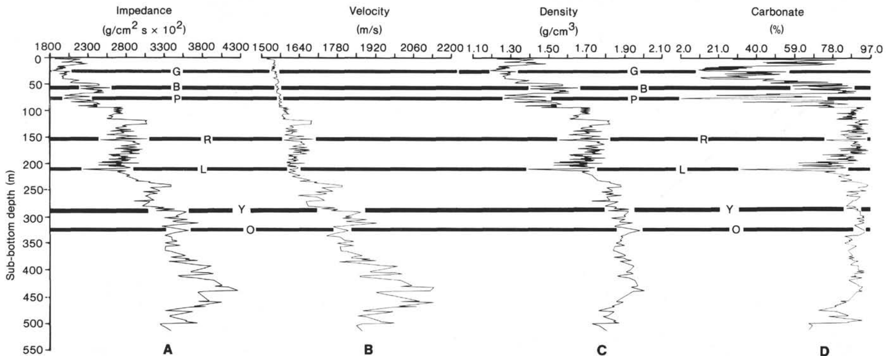
Figure 14. Correlation of major regional reflectors (G, B, P, R, L, Y, O) and physical properties at Site 574. A. Impedance versus sub-bottom depth, Site 574. B. Sonic velocity versus sub-bottom depth, Site 574. C. Saturated bulk density versus sub-bottom depth, Site 574. D. Percent carbonate versus sub-bottom depth, Site 574.
