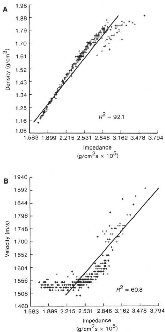
Figure 15. Correlation between density, velocity, and impedance. Solid line represents linear regression; R^2 = correlation coefficient. A. Regression of impedance against density, Site 574. B. Regression of impedance against velocity, Site 574.
