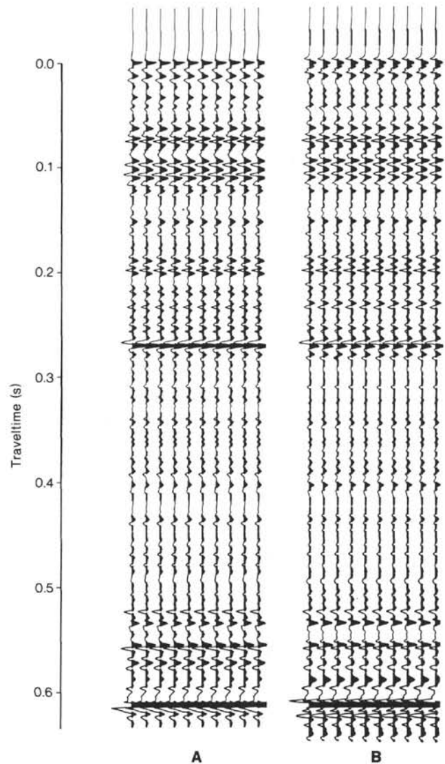
Figure 12. Calculated synthetic seismograms, DSDP Site 574. A. Deconvolved source signature. B. Raw source signature.
