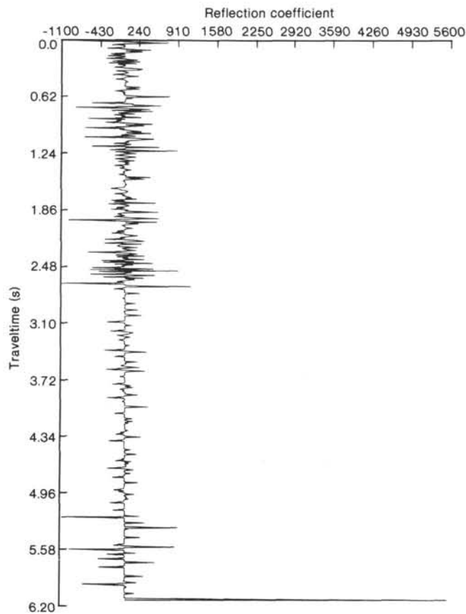
Figure 11. Reflection coefficient versus traveltime, DSDP Site 574.
