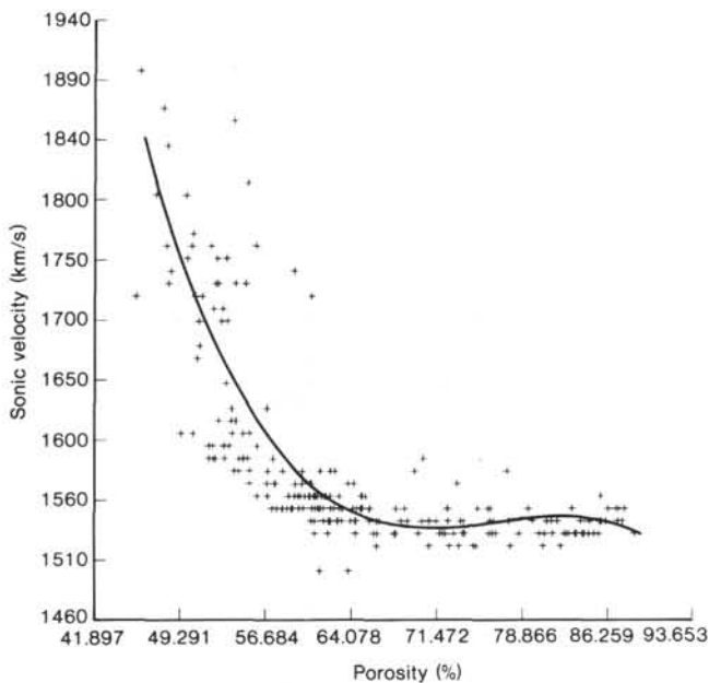
Figure 7. Regression of porosity against sonic velocity for DSDP Site 574. Solid curve is a third-order regression line.
