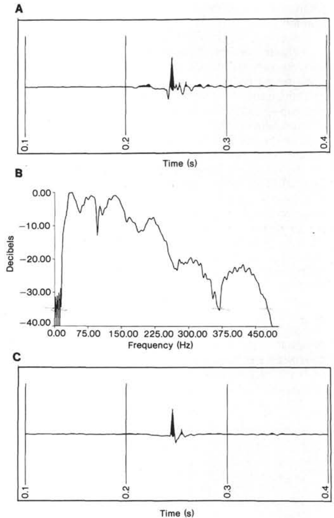
Figure 1. Source signatures for SIO 80-in. 3 watergun. A. Raw source signature. B. Spectrum of raw source signature. C. Source signature with DECONS operator applied.
