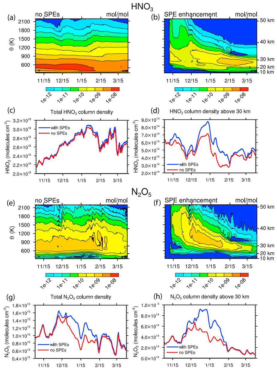
Figure 7. Time evolution of WACCM vortex-averaged (a) background HNO 3 (no SPEs), (b) SPE enhancement of HNO 3 (HNO 3 with SPEs – HNO 3 no SPEs), (c) total column density of HNO 3 , (d) column density of HNO 3 above 30 km, (e) background N 2 O 5 (no SPEs), (f) SPE enhancement of N 2 O 5 (N 2 O 5 with SPEs – N 2 O 5 without SPEs), (g) total column density of N 2 O 5 , and (h) column density of N 2 O 5 above 30 km.
