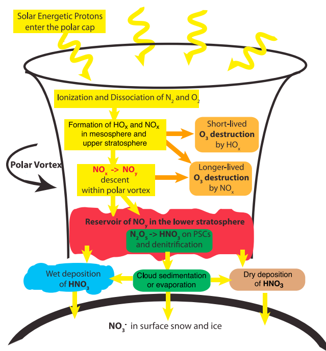
Figure 1. Schematic diagram of processes involved with nitrate deposition from solar energetic protons.
