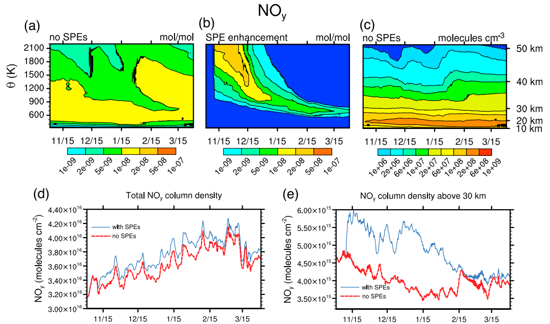
Figure 6. WACCM vortex-averaged NO y : (a) no SPEs (mole ratios), (b) SPE enhancements (mole ratios), (c) no SPEs (number density), (d) column densities (molecules cm -2 ) integrated throughout the total atmosphere with SPEs (blue) and no SPEs (red), and (e) column densities (molecules cm -2 ) integrate from 30 km to the top of the atmosphere with SPEs (blue) and no SPEs (red).
