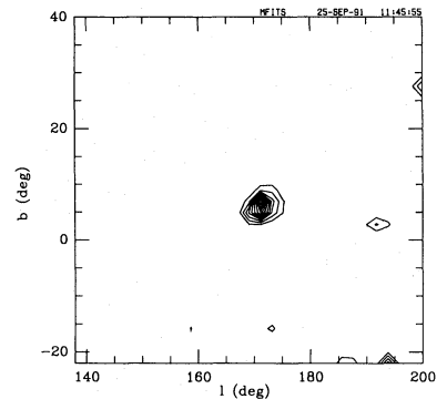
Fig. 8. Maximum entropy skymap of the GRB 910503 burst region. The contours are given in relative flux units.
