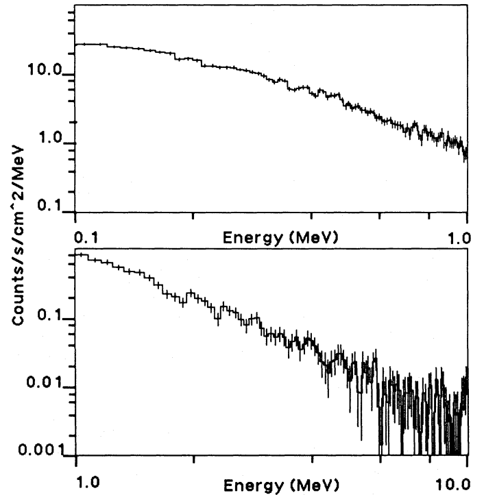
Fig. 6. Background subtracted count spectra for first pulse (top: low range, bottom: high range) obtained from COMPTEL's burst detectors.
