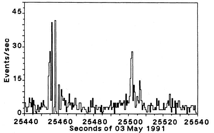
Fig. 2. GRB 910503: Lightcurve from COMPTEL imaging events. Data contain raw events without application of any selection criteria.
