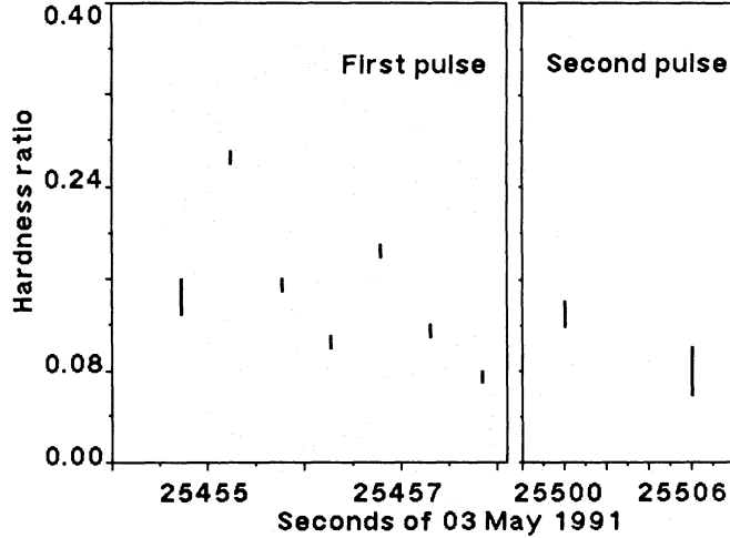
Fig. 4. Hardness ratio for both pulses of GRB 910503
