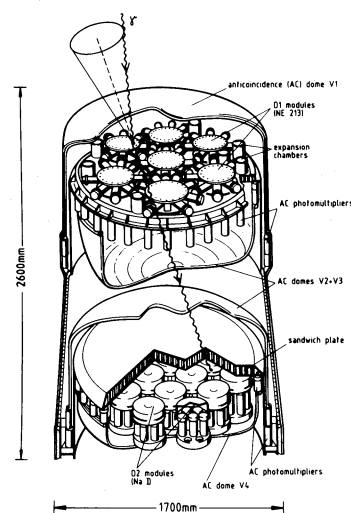
Fig. 1. Schematic view of COMPTEL
