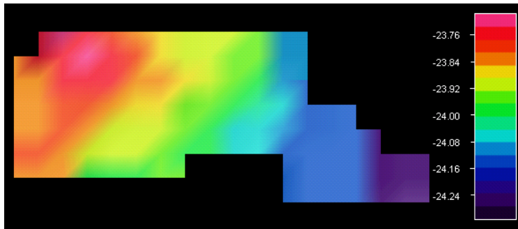
Figure 3a –ERZT MLLW SEP surface for NOAA H12216 [height in meters]
