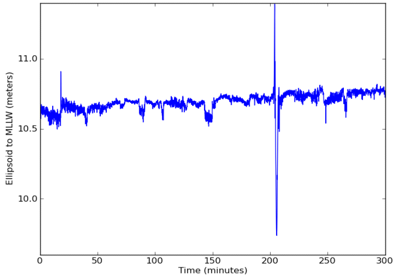
Figure 1 – Time series of ellipsoid to MLLW separation as estimated from one vessel with no filtering
