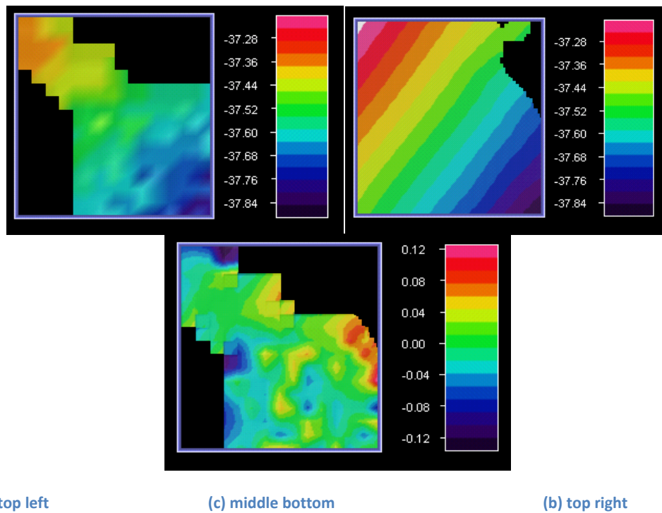
Figure 4 Depicts the area from NOAA survey H12180 with a vertical scale in meters. 3a is ERZT surface, 3b is the VDatum derived ellipsoid to MLLW surface, 3c is the ERZT and VDatum difference.
