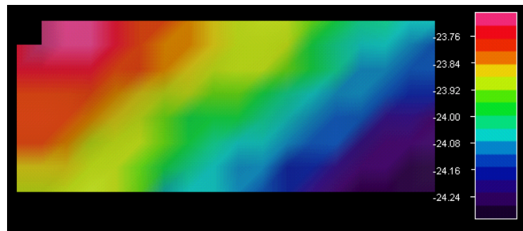
Figure 3b – VDatum MLLW SEP surface for NOAA H12216 [height in meters]
