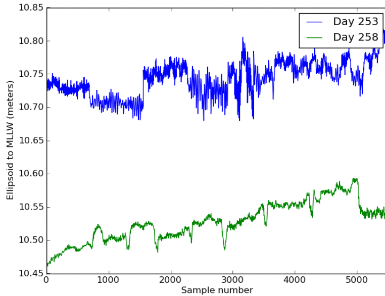
Figure 2 – Ellipsoid to MLLW separation estimates from the same survey vessel on two different days.
