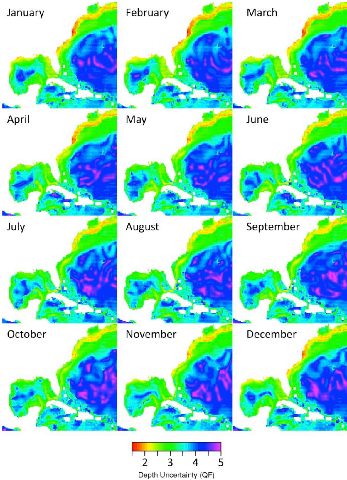
Figure 15. Monthly SVP Weather Maps derived from WOA2001 (1/4°) for Gulf of Mexico and U.S. Eastern seaboard.
