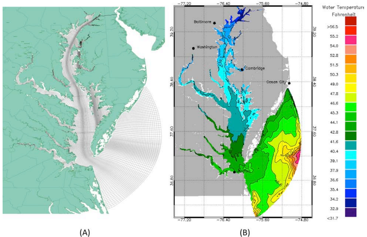
Figure 3. CBOFS model grid (A) and sample output of forecasted sea surface temperature (B). Salinity and sea surface height are also computed by the forecast system. Temperature and salinity are computed for 20 depth levels throughout the spatial domain of the model. Images (A) and (B) accessed from NOAA Tides and Currents website ( http://tidesandcurrents.noaa.gov/ofs/cbofs/ ).
