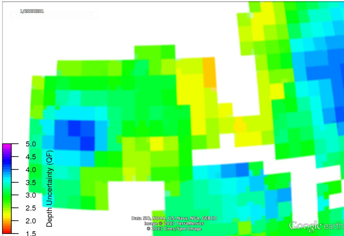
Figure 10. SVP Weather Map derived from WOA2009 1° model for February. Spatial resolution is 60NM.
