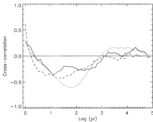
Fig. 7. Lagged cross-correlations. Solid curve shows correlation of observed \text{CO}_2 anomaly with temperature anomaly for positive lags (temperature leading \text{CO}_2 ). The remaining curves are for the optimized model with explicitly lagged N feedback (dotted line) and with no- N -feedback (dashed line).
