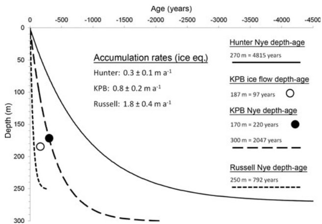
Fig. 11. Depth-age estimates for MH, KP and MR, calculated from models developed by Nye (1953) and Haefeli (1961). The black dot at 170 m depth represents the depth of SCS overlying complex strata imaged with GPR in KP. The open circle represents depth and age of SCS calculated from our flow model.
