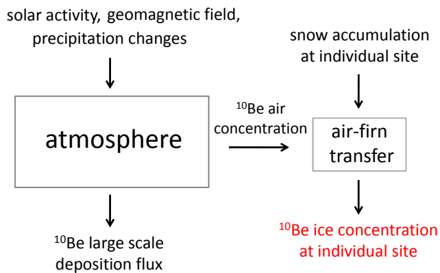
Figure 6. Sketch of our basic model approach to simulate ^{10}\text{Be} ice core records on the glacial–interglacial timescale. The model setup of the atmosphere is presented in Sect. 2.1, whereas the air–firm transfer model is put forward in Sect. 2.2. Model input records are discussed in Sect. 2.3.
