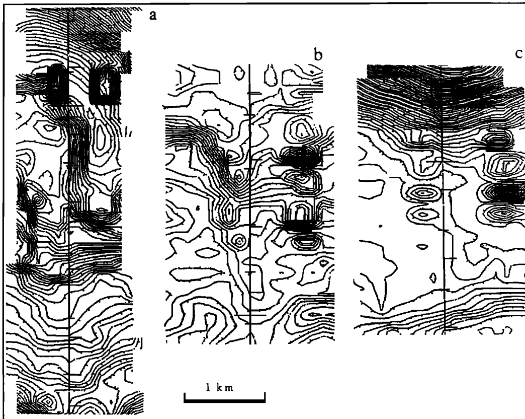
Fig. 8. Examples of contoured swath plots showing the results of external sound source interference. Artifacts can be recognized as individual peaks on one or both sides of the ship's track (center line in all three plots). Contour interval is 10 m, and tick marks point downhill.
