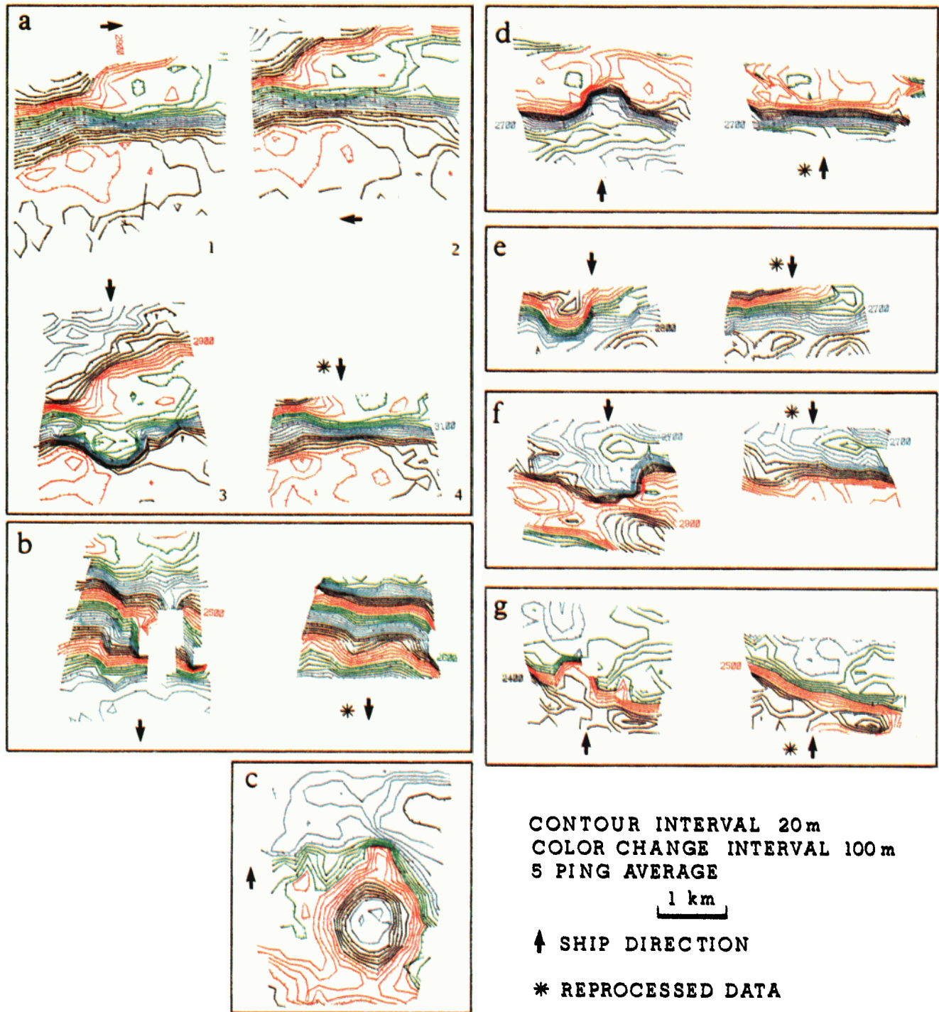
Plate 1. [de Moustier and Kleinrock] "Omegas" and gaps. Tick marks point downhill. Contoured sections not starred are original Sea Beam data. Contoured sections marked with a star are the result of reprocessing the acoustic data recorded digitally with the MPL system. Our simplified echo-processing technique does not include ray-bending corrections, and arrival times are determined by the first arrival above a preset threshold. The threshold level is selected after visual inspection of the roll-compensated acoustic data. Recomputed depths and cross-track distances are therefore in uncorrected meters referenced to a sound velocity of 1500 m/s. Although crude, this processing method suffices to prove the fictitious character of Sea Beam's contoured bathymetry shown in Plates 1a, (section 3), 1b, 1d, 1e, 1f and 1g. We do not show a recomputed version of Plate 1c because the corresponding acoustic data was only recorded every five pings. This was enough to confirm the "omega" effect, but contour resolution was seriously degraded by the five ping decimation.
