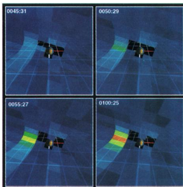
Figure 4. Substorm-associated ENA emissions on July 31, 1996. Polar is in the dawn sector and noon is to the right.
