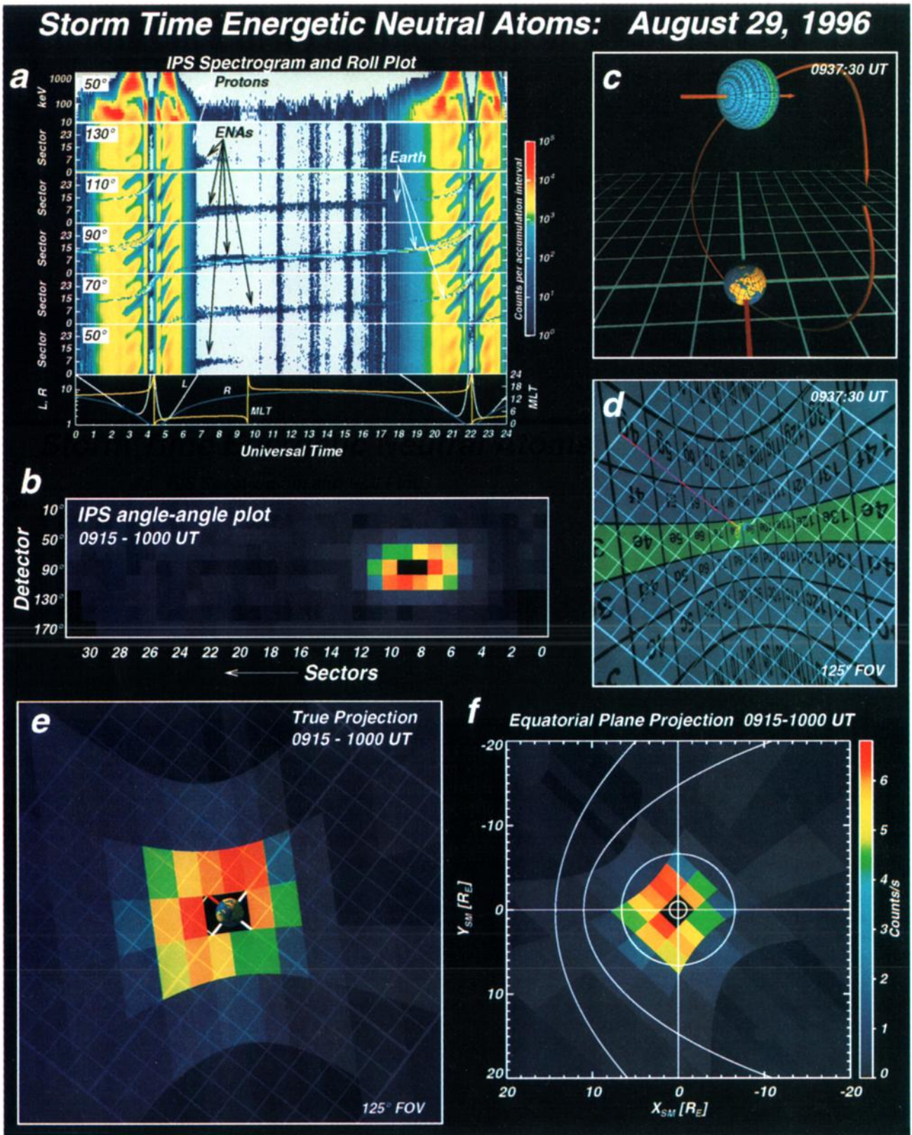
Figure 2. Storm-time ENA imaging on August 29, 1996. In (a), the IPS spectrogram from the 50° detector is shown along with the (integral energy channel) sector vs. time plots from the 50°, 70°, 90°, 110°, and 130° detectors. An angle-angle plot (i.e. a polar-angle versus azimuthal-angle plot) constructed from this data is shown in (b). (c) shows the attitude and location of Polar in its orbit at 0937:30 UT in the solar magnetic coordinate system. The white mesh represents the SM X-Y plane and the positive x-axis is marked with a red line. The view that IPS (and each of the individual sectors) has of the Earth at 0937:30 UT is shown in (d). The final two panels show the resulting ENA image in a true projection (e) and in an equatorial SM plane projection (f).
