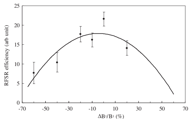
FIG. 11. The spin-flip efficiency of the RFSR is shown as a function of a relative change in the rf field \Delta B_1/B_1 . This spin-flip efficiency measurement with cold neutrons is based on the well-known parity-violating \gamma -ray asymmetry on ^{35}\text{Cl} at cold neutron energies (see text). The solid line is a fit to a quadratic function.
