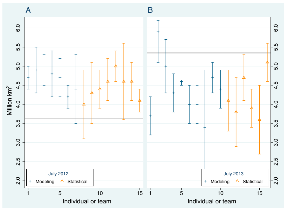
Figure 2. Predictions with contributor-supplied uncertainty from Sea Ice Outlook in (a) July 2012 and (b) July 2013, shown with the observed September ice extent (gray line).
