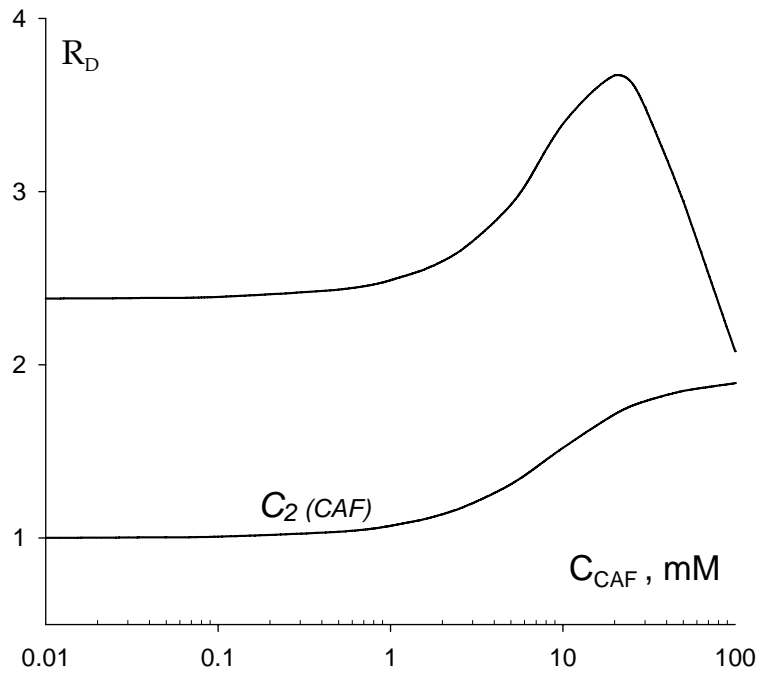
Fig.7 Relation between R_D , a measure of the effectiveness of the interceptor and protector action of Caffeine, and the concentration of CAF; C_{2(CAF)} is a schematic depiction of the absolute concentration of CAF-tetramer complexes
