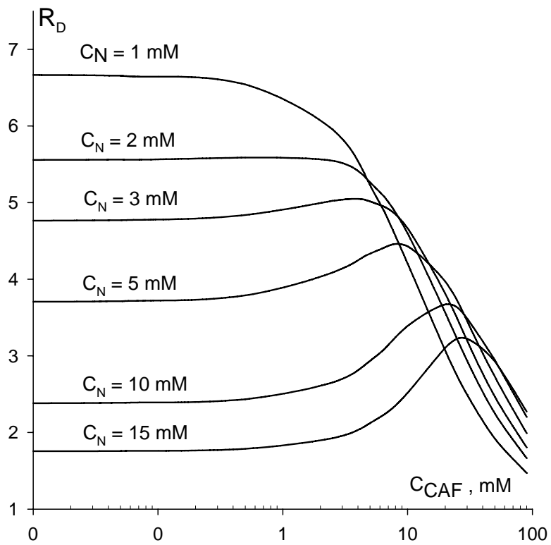
Fig.8 Relation between R_D , a measure of the effectiveness of the interceptor and protector action of Caffeine, and the concentration of CAF for different concentrations of nucleotide ( C_N ).
