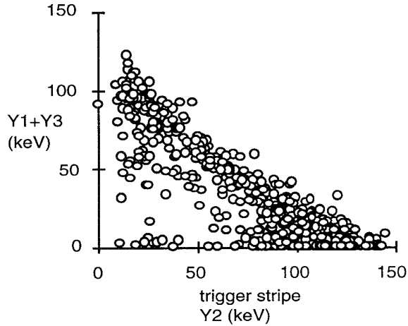
Figure 4b. Event-by-event distribution illustrating ^{57}\text{Co} signal sharing between the trigger stripe, Y2, and its neighbors
