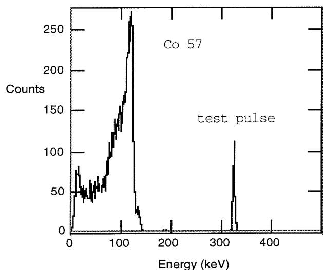
Figure 2. ^{57}\text{Co} response. Single stripe, ungated by coincidence with a stripe in the orthogonal dimension. 26 mm length, 0.375 mm width.
