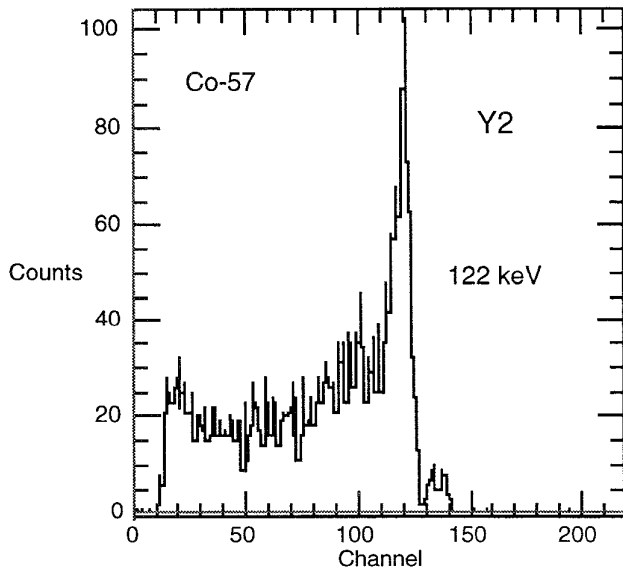
Figure 5a. 3355 ^{57}\text{Co} events. Distribution of trigger stripe (Y2) pulse height only. Single "pixel" defined by X2-Y2 coinc.
