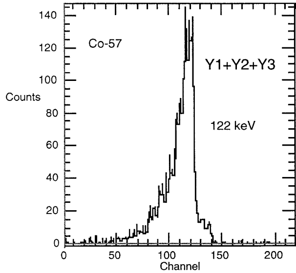
Figure 5b. Same 3355 ^{57}\text{Co} events. Distribution of sum of pulse heights, trigger stripe plus adjacent stripes.
