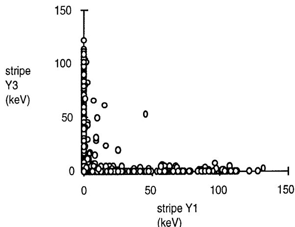
Figure 4a. Event-by-event distribution of ^{57}\text{Co} signal among stripes adjacent to the coincidence trigger stripe, Y2
