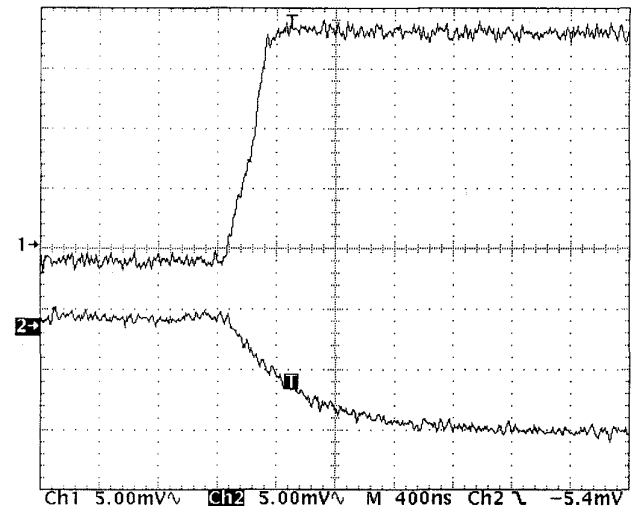
Figure 8. Charge sensitive preamplifier (Ortec model 142A, inverting) outputs for coincident electron (upper trace) and hole (lower trace) signals. Time scale is 400 n.sec/div.
