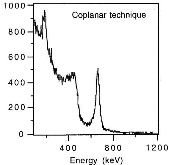
Figure 6. ^{137}\text{Cs} response. Spectrum from eight consecutive stripes of the prototype strip detector operating in coplanar grid mode. FWHM: 39 keV at 662 keV.
