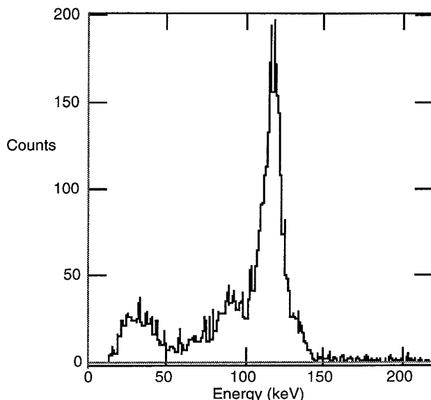
Figure 3. ^{57}\text{Co} response. Single "pixel", 0.375 \times 0.375 mm, defined by X-Y coincidence. FWHM: 9.8 keV at 122 keV (test pulse 5.5 keV, not shown).
