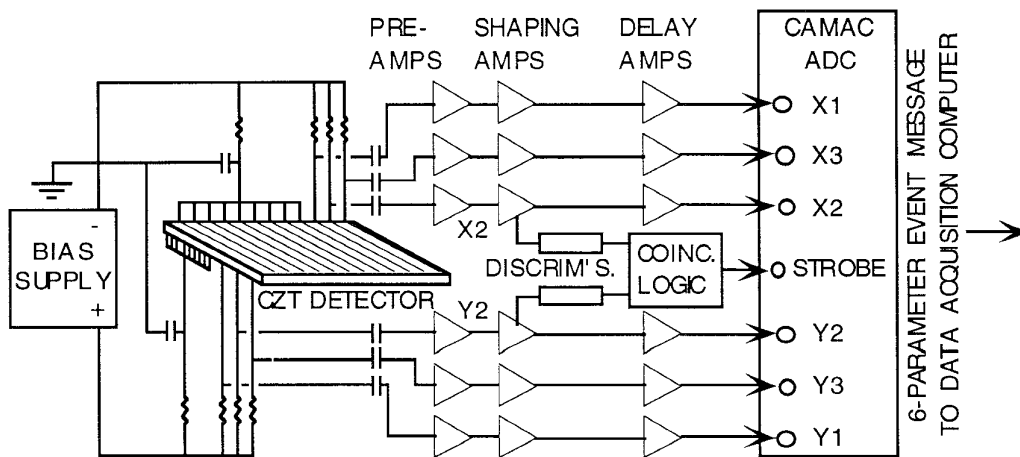
Figure 1. Test setup (orthogonal stripe coincidence mode)
