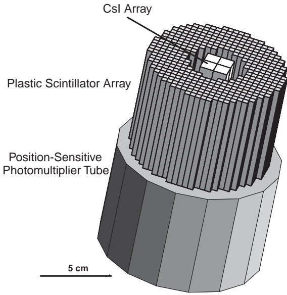
FIGURE 1. Schematic diagram of a polarimeter module.
