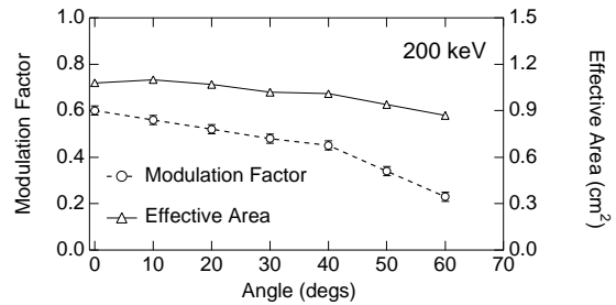
FIGURE 3. The effective area and modulation factor as a function of incidence angle for 200 keV photons (from simulations).
