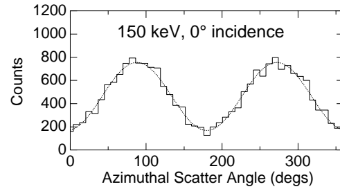
FIGURE 2. The simulated polarimetric response of a GRAPE module. Polarized 150 keV photons vertically incident on the module show an asymmetry in the azimuthal distribution of interactions in the plastic array. The data here have been corrected for intrinsic asymmetries in the module geometry.
