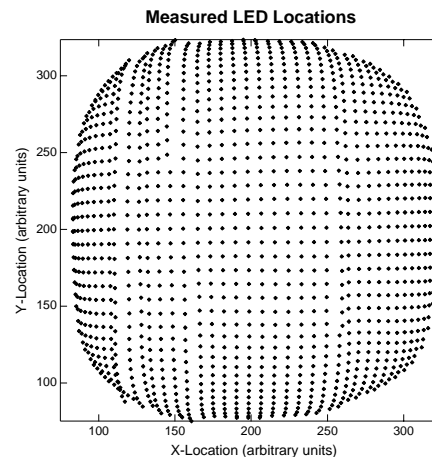
FIGURE 5. Plot of the measured (relative) positions of the LED calibration points.
