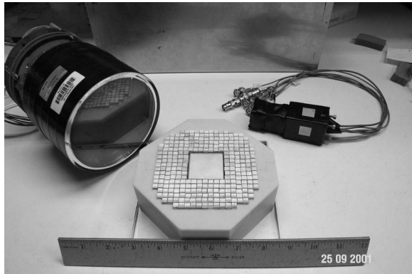
FIGURE 4. The components of the laboratory science model, showing (left to right) the PSPMT, the array of plastic scintillators, and the MAPMT/CsI assembly that fits into the central well of the plastic array.
