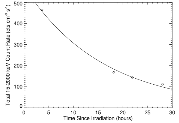
Fig. 15. Total internal counting rate (15-2000 keV) due to activation in \text{LaCl}_3 for a proton fluence equivalent to 5 years of SAA passages.
