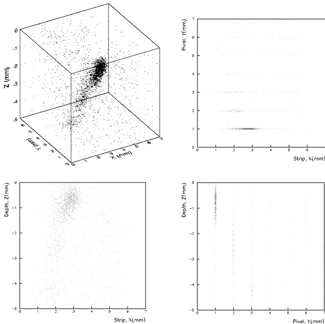
Fig. 11. Beam spot image, \sim 25^\circ incidence. 3-d event locations (top left), projections (clockwise) xy , xz and yz . Note: cathode is at Z=0 ; sign of Z was inverted to facilitate the graphic illustration.
