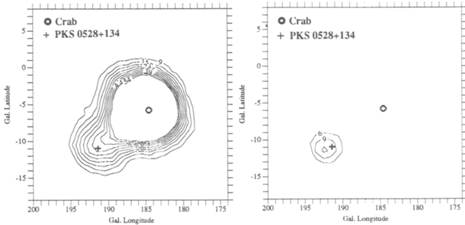
Fig. 1. Maximum-likelihood skymaps of the Crab region in the 10-30 MeV band from combined VP 0, 1, 213. Fig. 1a shows the Crab and the evidence for PKS 0528+134. Crab dominates the map. The likelihood ratio contours start at a value of 9 with a step of 5, and are cut off at a value of 54. Fig. 1b shows the likelihood map of the same region with the Crab removed (a model of the Crab was included in the null hypothesis of the likelihood fitting procedure). The remaining feature is evidence for PKS 0528+134.
