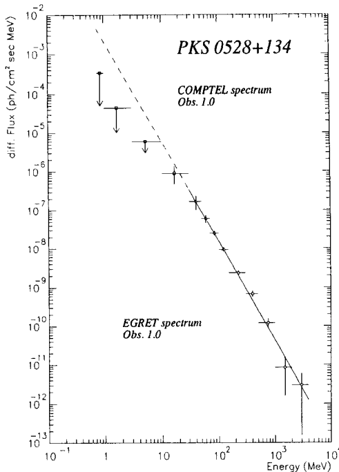
Fig. 3. Contemporaneous COMPTEL and EGRET energy spectra of PKS 0528+134 during VP 1. The COMPTEL upper limits are 2\sigma . The EGRET spectrum is from Hunter et al. (1993). The dashed line represents the extrapolation of the EGRET spectrum throughout the COMPTEL energy range. The evidence for a spectral break is visible.
