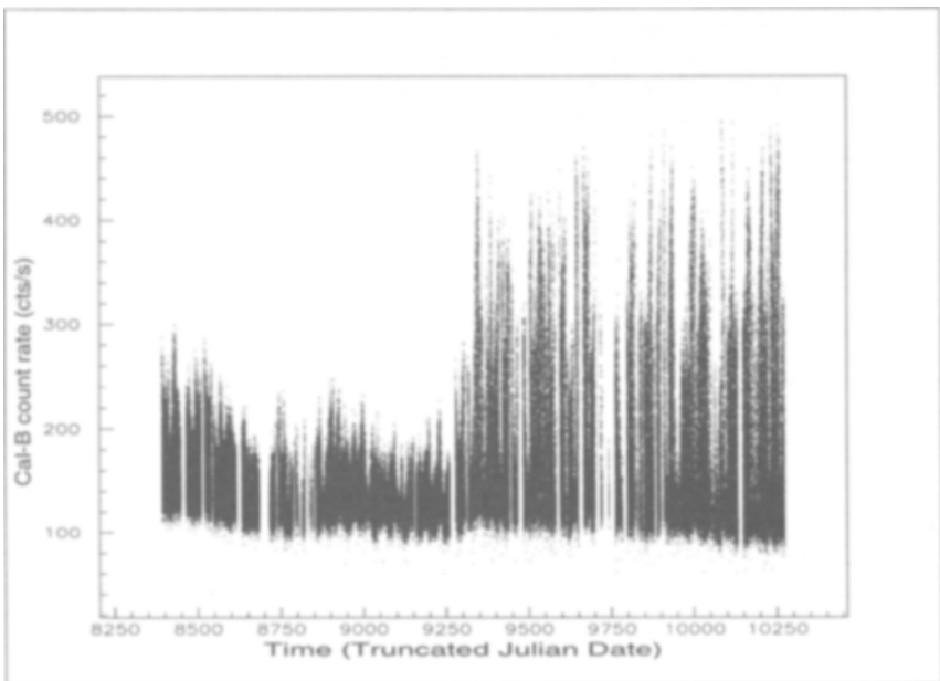
FIGURE 1. Measured count rates of Cal-unit B as a function of time.
