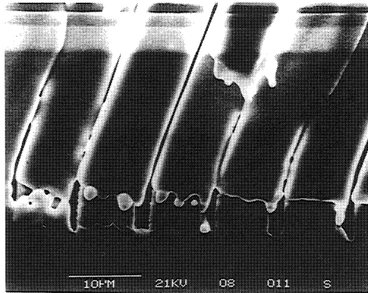
Figure 2. SEM closeup view of 300µm film. The substrate pattern can be seen clearly at the bottom of the columns, with the well-separated CsI fibers growing up from the tops of the substrate pedestals.
