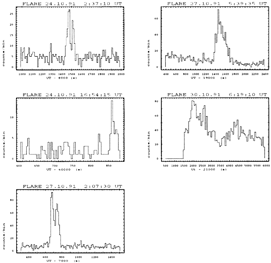
Figure 1. Time profiles of solar flares detected in COMPTEL telescope mode.
