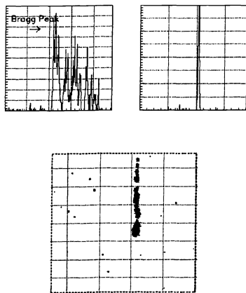
Fig. 16. 1-d projections (top) of 2-d proton track image from the SONTRAC Science Model.
