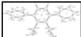
Fig. 1. The molecular structure showing the crystallographic labeling scheme and displacement ellipsoids drawn at the 50% probability level. H atoms are shown as spheres of arbitrary radii.
