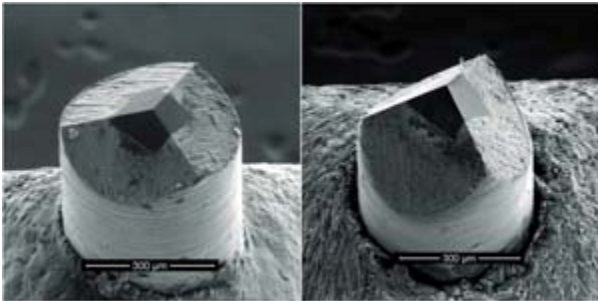
Figure 4: The Berkovich indenter tip (left) and the Cube Corner indenter tip (right). (University of Nebraska-Lincoln, College of Engineering)
