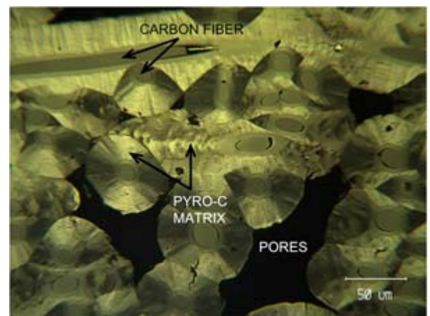
Figure 3: A micrograph of the structure of the carbon-carbon composite tested, showing the Pyro-C matrix surrounding the carbon fibers and the pores that are formed during deposition.
