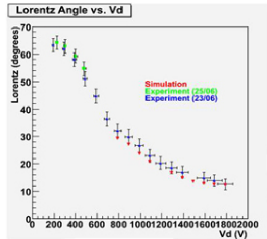
BOTTOM RIGHT: Fig. 8 – Plot showing observed Lorentz angle versus drift voltage. In this plot, there are two runs of experimental data and one of simulated data superimposed in different colors. In these experiments, the magnetic field strength was constant.
