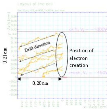
Fig. 4 – Data from CERN simulations under normal laboratory conditions in CLAS12. (3)
