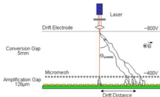
Fig. 5 – Experimental setup used to study the Lorentz angle. (4)
