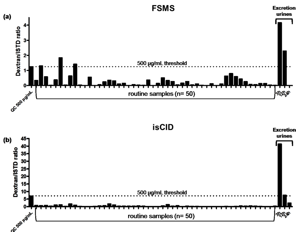
FIG. 6. SEMI-QUANTITATIVE DETERMINATION OF [Glu_3-H_2O+H]^+ CONCENTRATION IN A REPRESENTATIVE BATCH OF ROUTINE SAMPLES (N= 50), COMPARED TO A QUALITY CONTROL SAMPLE SPIKED AT 500 \mu\text{g} \cdot \text{mL}^{-1} IN FSMS (A) AND ISCID (B) MODE AND 3, 12 AND 24 HOURS EXCRETION SAMPLES.
