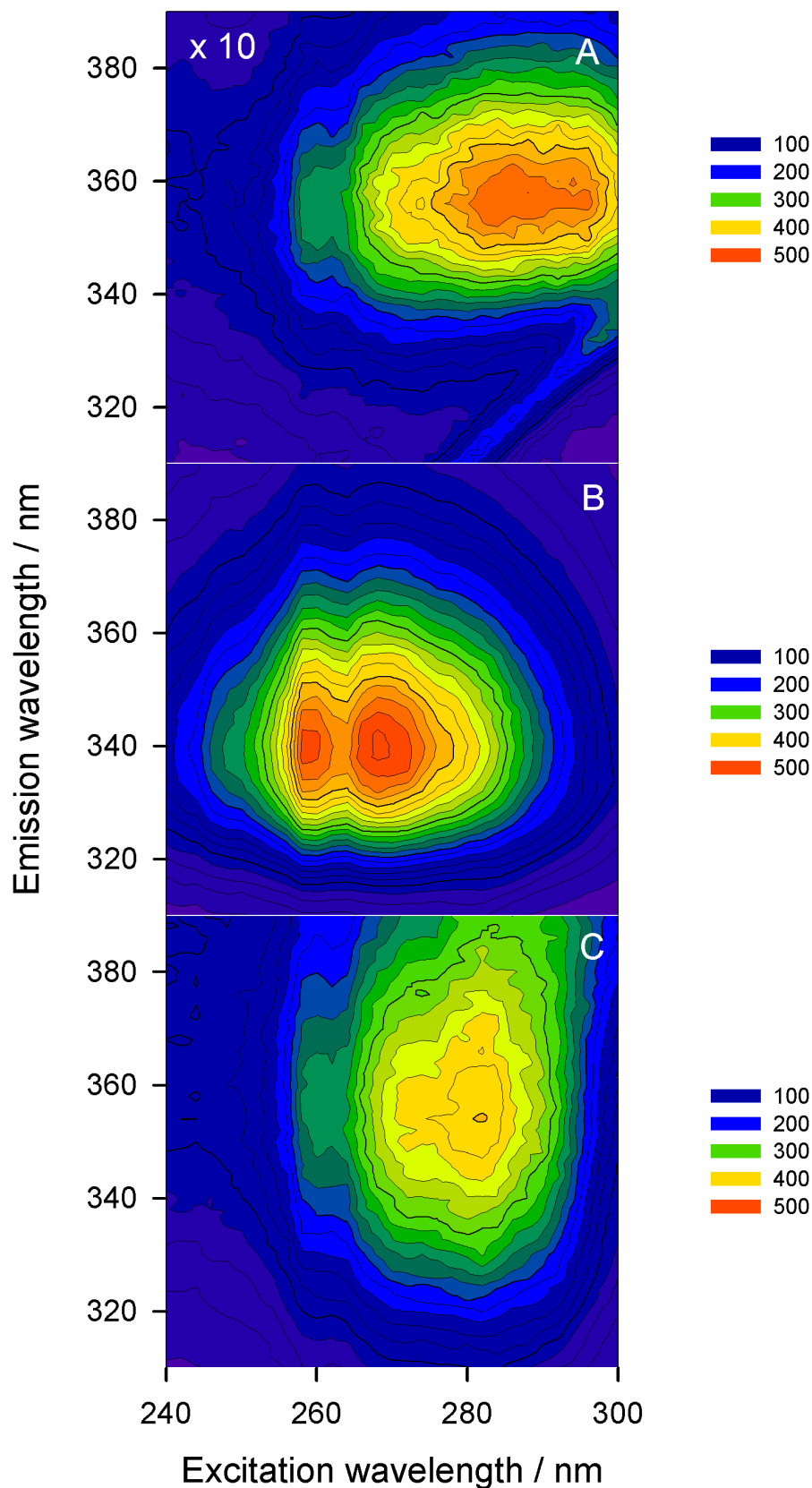
Figure 1. A) Contour plot of the excitation-emission matrix of a solution of PRO ( 900 \text{ ng mL}^{-1} ) at \text{pH} = 5.0 to avoid hydrolysis. The intensities have been multiplied by a factor of 10. The coloured bar on the right shows the fluorescence intensities. B) Contour plot of the EEM for a 500 \text{ ng mL}^{-1} solution of PAB at \text{pH} = 13 . C) Contour plot of the EEM for a typical equine serum, after deproteinization and 1:20 dilution at \text{pH} = 13 . Notice the higher fluorescence intensities of PAB and serum in comparison with PRO.
