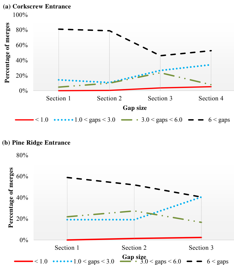
Figure 4.5. Merge percentage vs. gap size offered by freeway traffic.
