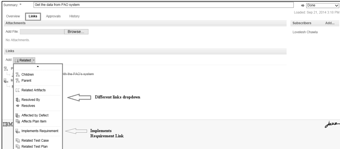
Figure 18. Links Tab
