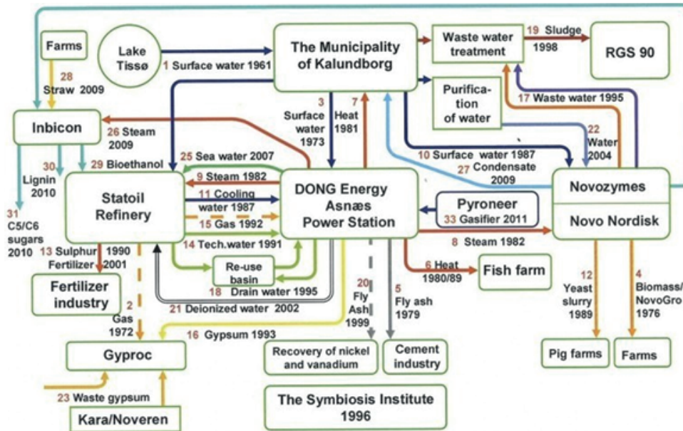
Figure 1. The system of industrial symbiosis in Kalundborg
