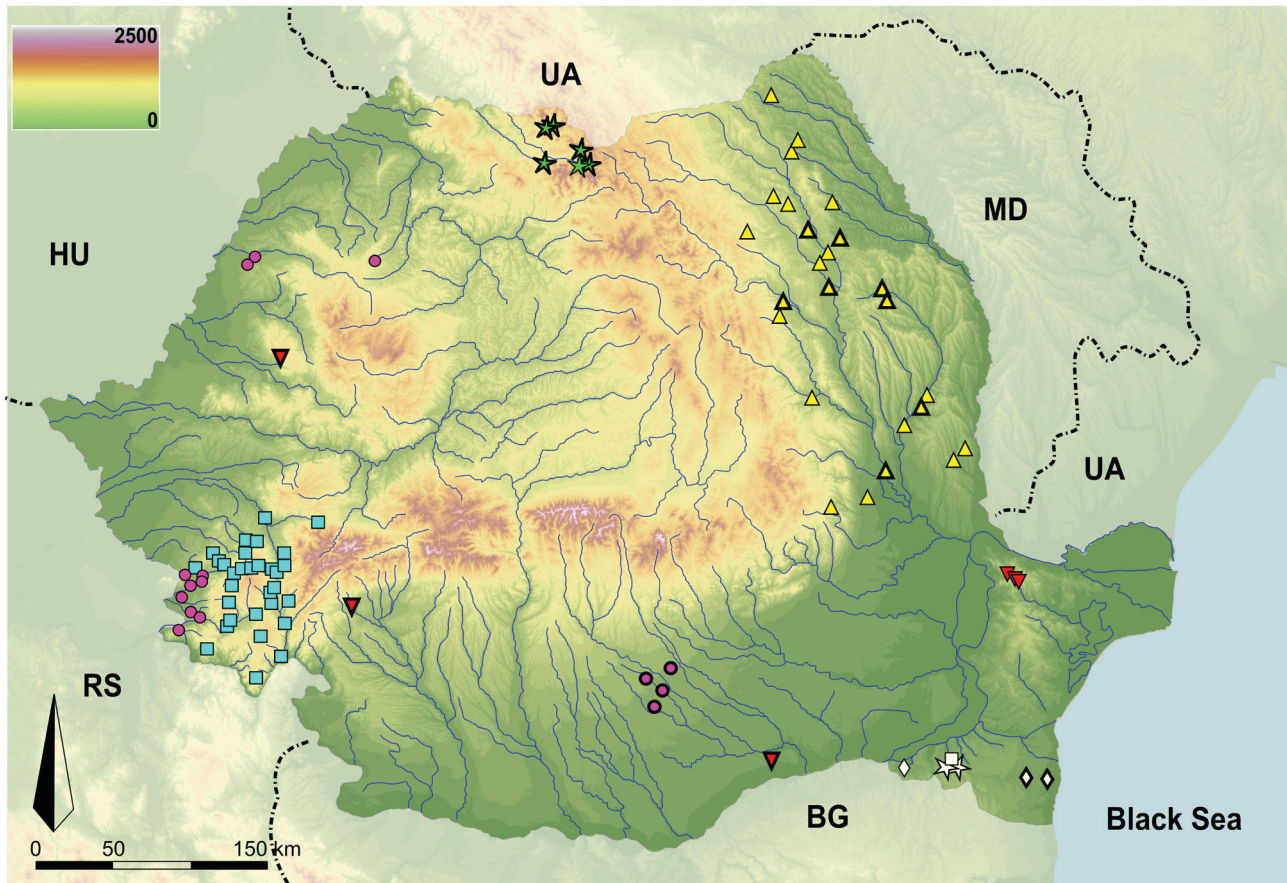
FIGURE 2. Distribution of G. arduus (red downward pointing triangles), G. kischineffensis (yellow upward pointing triangles), G. cf. kischineffensis (turquoise squares), G. komareki s.l. (white square), G. leopoliensis (green stars), G. pulex s.l. (white diamonds), and G. roeselii s.l. (pink circles) in Romania. White stars represent localities where G. komareki s.l. and G. pulex s.l. coexist. Shapes with thin outline—data from this study, shapes with thick outline—data from the literature. For country abbreviations, see Fig. 1.
