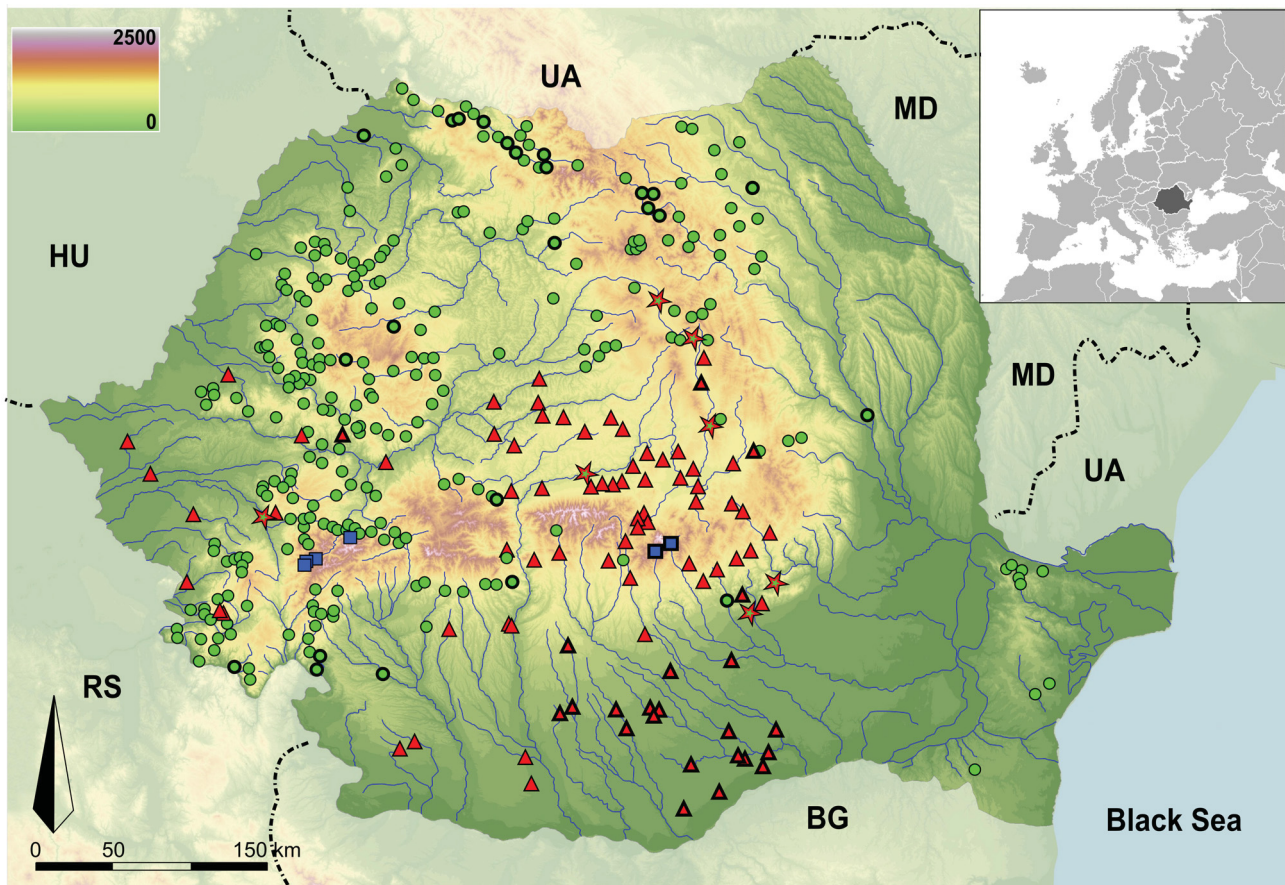
FIGURE 1. Distribution of G. cf. balcanicus (green circles), G. b. dacicus (red triangles) and G. b. montanus (blue squares) in Romania. Stars represent localities where G. cf. balcanicus and G. b. dacicus coexist. Shapes with thin outline—data from this study, shapes with thick outline—data from the literature. Countries are indicated by their 2-letter ISO codes: HU—Hungary, UA—Ukraine, MD—Republic of Moldova, BG—Bulgaria and RS—Serbia.
