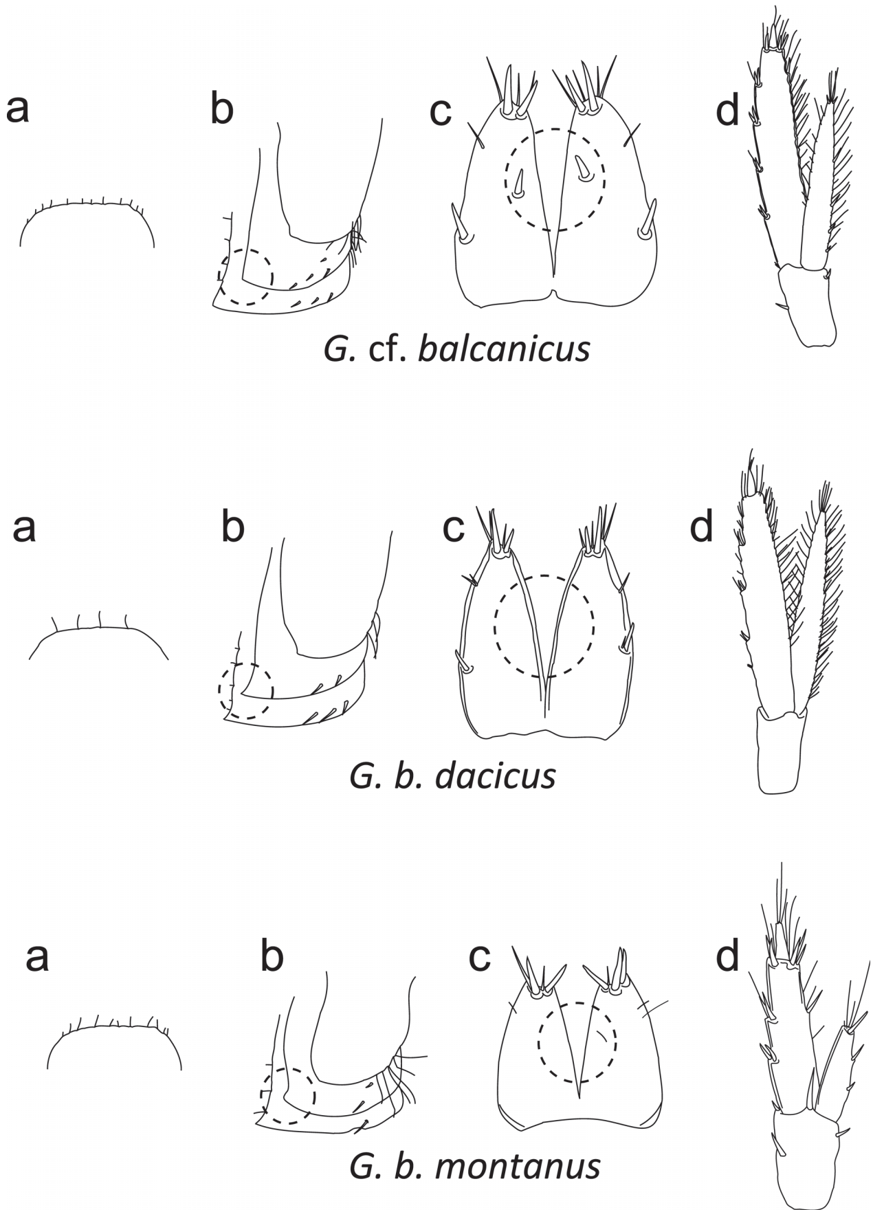
FIGURE 6. Main morphological differences between the three morphs of G. balcanicus . a) dorso-posterior side of metasome segment 3, b) epimeral plates, c) telson, d) third uropod.
