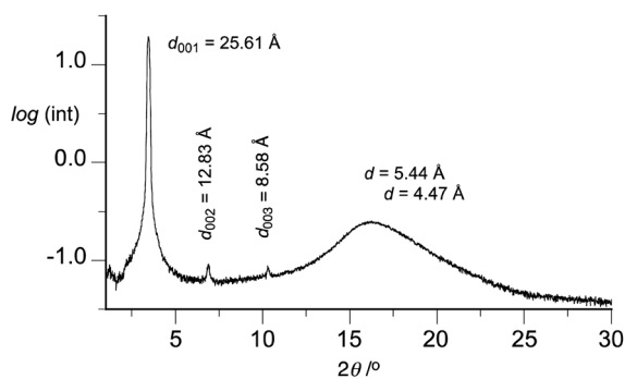
Fig. 5 XRD pattern for 2[10]b at 195^{\circ}\text{C} .
