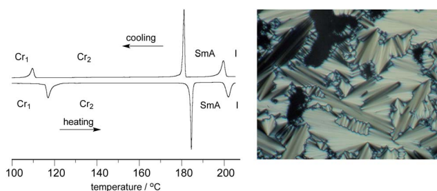
Fig. 4 (Left) DSC trace of 2[10]b . The heating and cooling rates are 5 \text{ K min}^{-1} . (Right) The optical texture of 2[10]b obtained at 190^{\circ}\text{C} on cooling from the isotropic phase.
