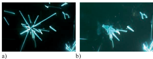
Fig. 4 Optical textures observed for 1[10]d in the same region of the sample: (a) Col h phase at 78 ^{\circ}\text{C} and (b) Col h(3D) phase at 70 ^{\circ}\text{C} . The exposure times are 1/8 s for (a) and 1/3 s for (b).
